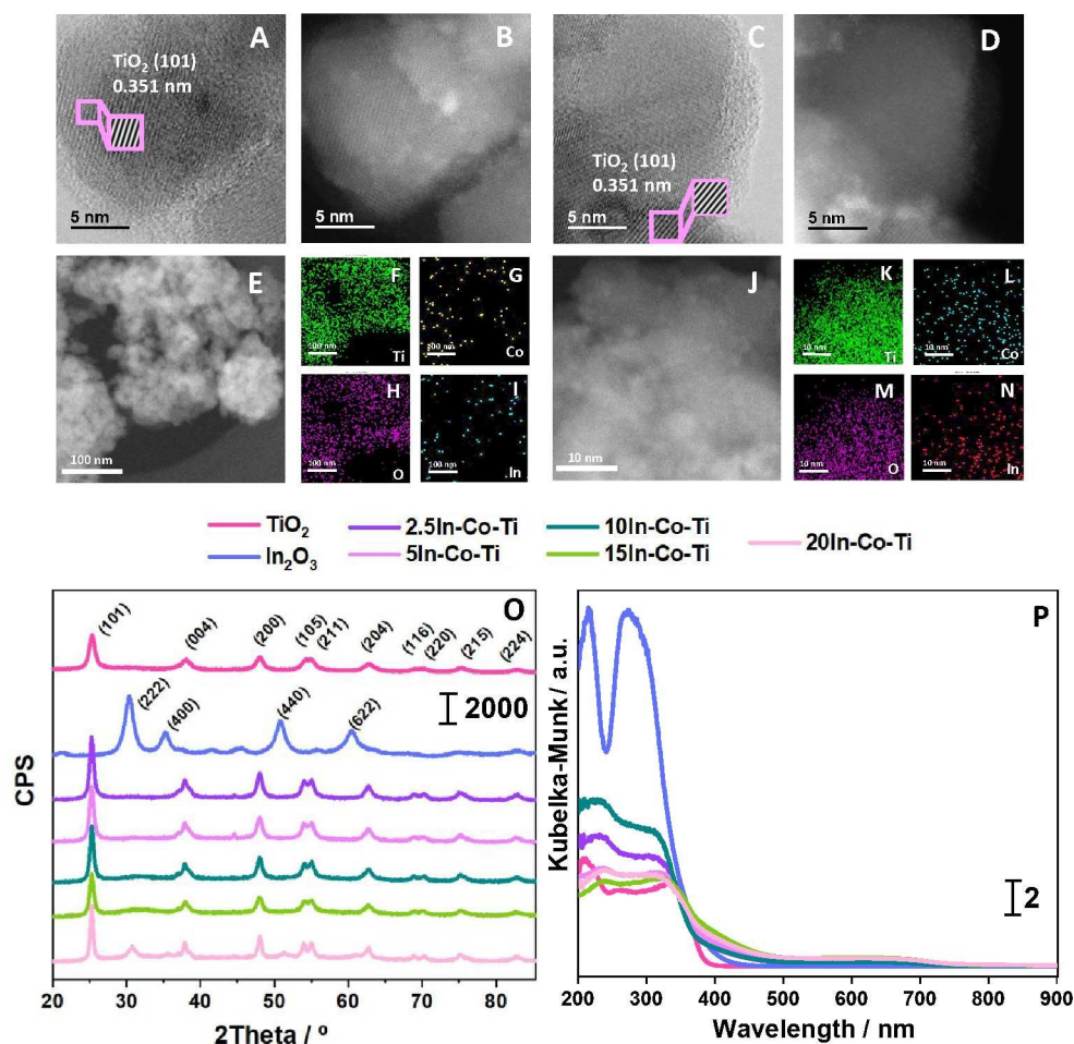
Figure 2. (A,B) TEM micrographs for the 2.5In-Co-Ti sample. (C,D) TEM Micrographs for the 10In-Co-Ti sample. (E-I) Dark-field STEM (E) and EDS mapping for the 2.5In-Co-Ti sample. (J-N) Dark-field STEM (J) and EDS mapping for the 10In-Co-Ti sample. (O) XRD patterns for the xIn-Co-Ti and reference samples. (P) UV-visible plot spectra for the xIn-Co-Ti samples.
