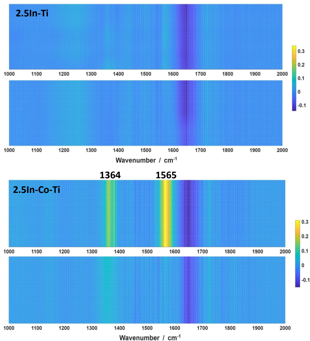
Figure 8. In situ infrared results for the 2.5In-Co-Ti sample and 2.5In-Ti reference obtained under reaction conditions at 250 °C. For each material, the lower panel corresponds to results obtained under thermal excitation while the upper panel displays results under photothermal conditions.
