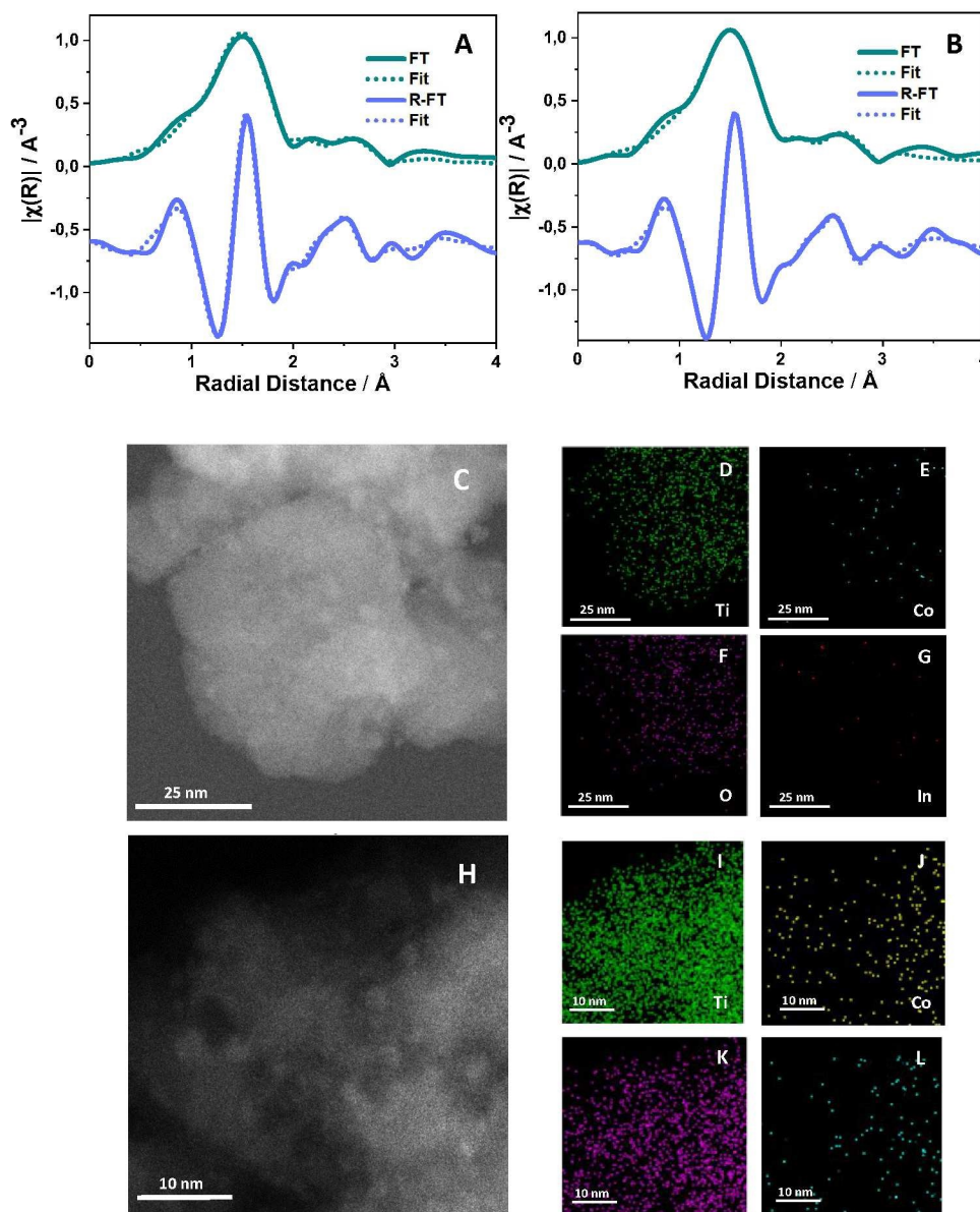
Figure 6. K 2 -weighted real part (R-FT) and module (FT) of the Fourier transform of the Co K-edge EXAFS signal for the 2.5In-Co-Ti sample after thermal reaction at 250°C. (B) K 2 -weighted real part (R-FT) and module (FT) of the Fourier transform of the Co K-edge EXAFS signal for the 2.5In-Co-Ti sample after photothermal reaction at 250°C. Experimental (R-FT, FT) and fitting results are presented. (C-G) Dark-field STEM (C) and EDS mapping for the 2.5In-Co-Ti sample after thermal reaction at 250°C. (H-L) Dark-field STEM (H) and EDS mapping for the 2.5In-Co-Ti sample after photothermal reaction at 250°C.
