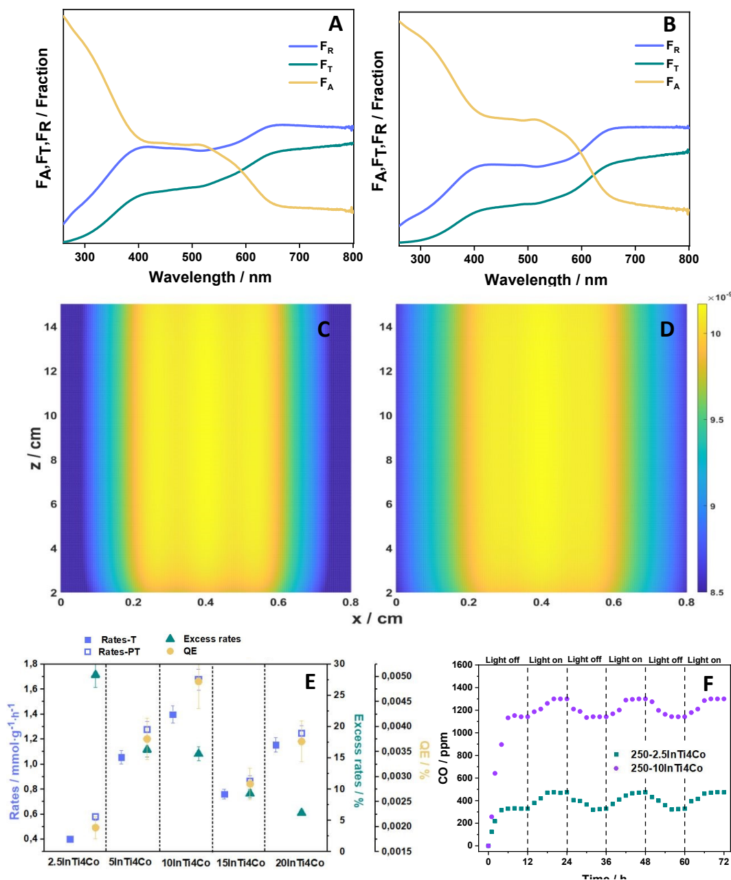
Figure 5. (A-B) Fraction of light absorbed, transmitted or reflected by the 2.5In-Co-Ti and 10In-Co-Ti samples, respectively. (C-D) Local photon absorption rate at 250 °C ( \text{Einstein m}^{-2} \text{s}^{-1} ) under irradiation for the 2.5In-Co-Ti and 10In-Co-Ti samples, respectively. (E) Reaction rates, excess rates and quantum efficiency for xIn-Co-Ti samples. (F) Long-term operation tests for selected samples under light off/on cycling conditions.
