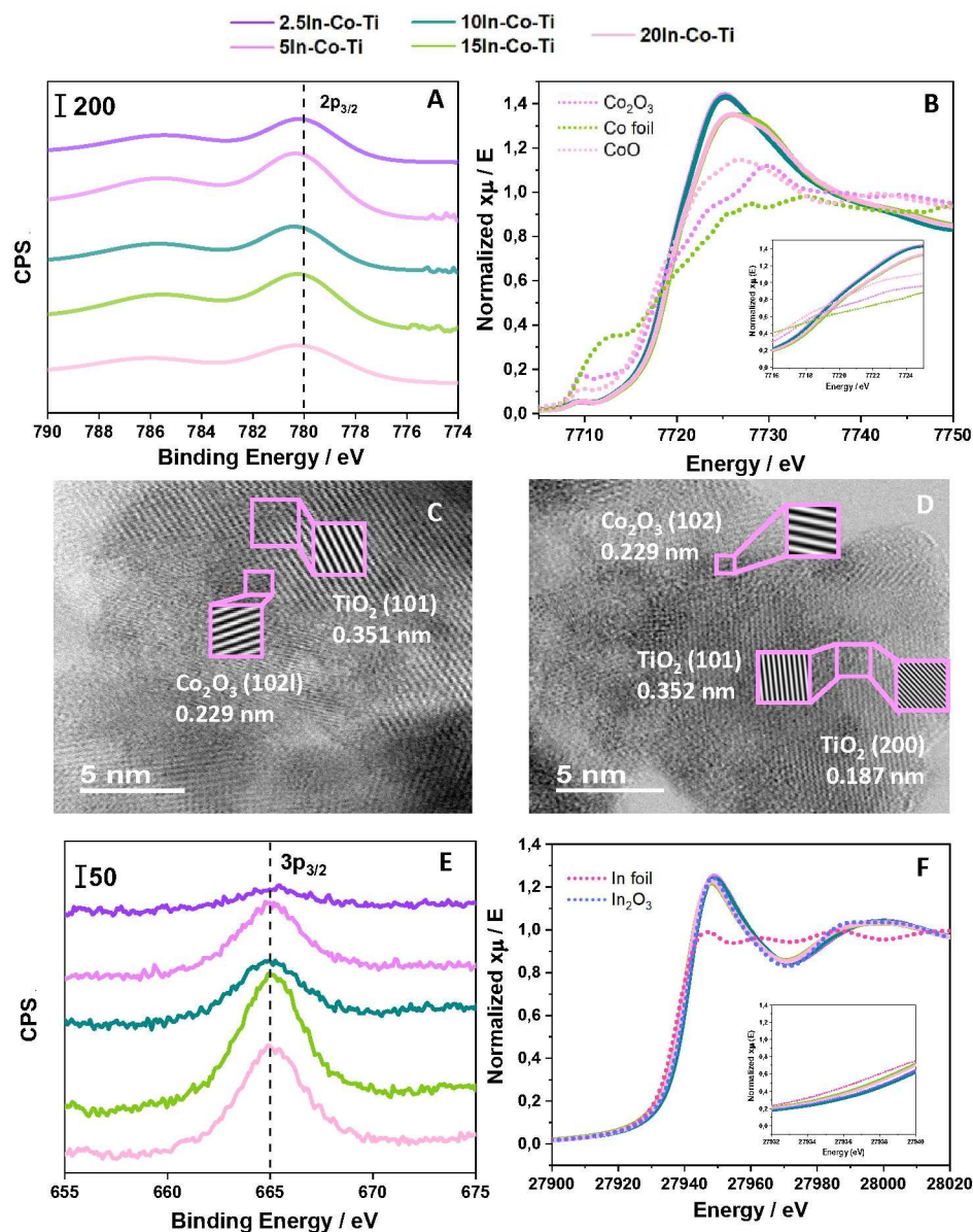
Figure 3. (A) Co 2p 3/2 XPS spectra for the xIn-Co-Ti samples. (B) Co K-edge XANES spectra for the xIn-Co-Ti catalysts and reference samples. (C) TEM micrographs for the 2.5In-Co-Ti sample. (D) TEM Micrographs for the 10In-Co-Ti sample. (E) In 3p 3/2 XPS spectra for the xIn-Co-Ti samples. (F) In K-edge XANES spectra for the xIn-Co-Ti catalysts and reference samples.
