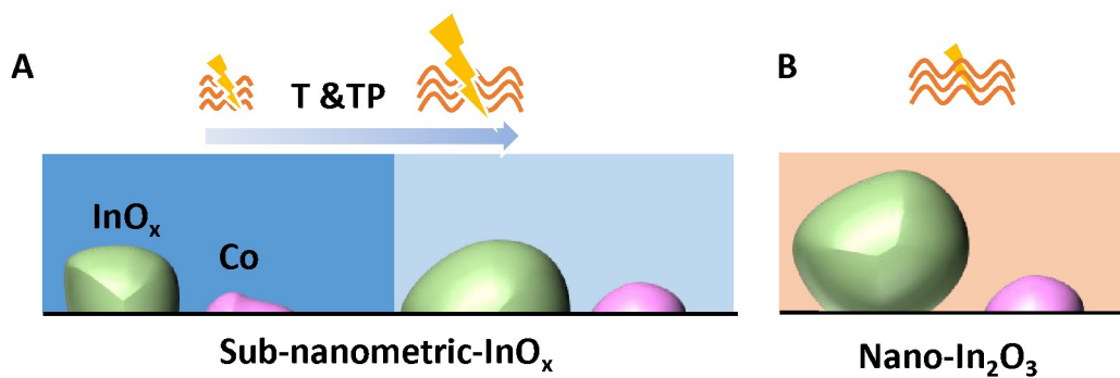
Figure 9. Schematic representation of the photothermal effects and local structure of cobalt and indium species for (A) 2.5-15In-Co-Ti and (B) 20In-Co-Ti samples.
