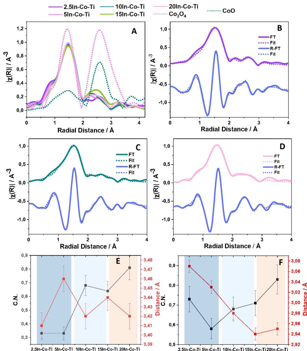
Figure 4. (A) k^2 -weighted Fourier Transform (FT) of the Co K-edge EXAFS signal for the catalysts and reference samples (B-D) Real part (R-FT) and module (FT) of the Fourier transform for selected samples. Experimental signals (R-FT, FT) and fitting results are presented. (E) Coordination number (C.N.) and distance of the Co-Co shell for the xIn-Co-Ti samples. (F) Coordination number (C.N.) and distance of the Co-Ti shell for the xIn-Co-Ti samples.
