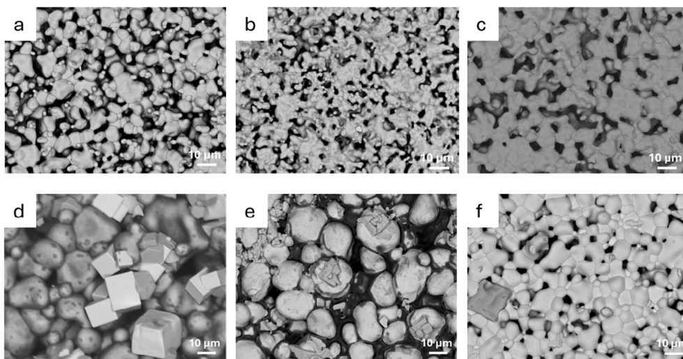
Fig. 16 Backscattered electron detector (BSED) SEM images of the base pellets in contact with alumina crucible sintered at 900 °C (a) \text{Li}_5\text{La}_3\text{Nb}_2\text{O}_{12} , (b) \text{Li}_5\text{La}_3\text{NbTaO}_{12} , and (c) \text{Li}_5\text{La}_3\text{Ta}_2\text{O}_{12} and 1100 °C (d) \text{Li}_5\text{La}_3\text{Nb}_2\text{O}_{12} , (e) \text{Li}_5\text{La}_3\text{NbTaO}_{12} , and (f) \text{Li}_5\text{La}_3\text{Ta}_2\text{O}_{12} . Increased density was observed at 1100 °C.
