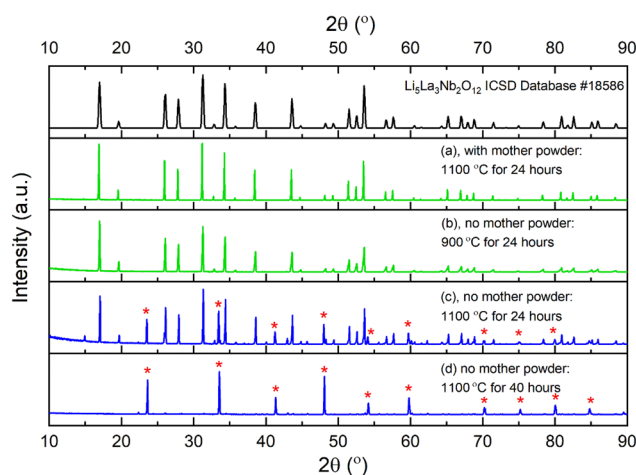
Fig. 15 Ex situ PXRD patterns of \text{Li}_5\text{La}_3\text{Nb}_2\text{O}_{12} pellet in contact with alumina crucible during sintering at (a) 1100\text{ }^\circ\text{C} for 24 hours with sacrificial mother powder, (b) 900\text{ }^\circ\text{C} for 24 hours without mother powder, (c) 1100\text{ }^\circ\text{C} for 24 hours without mother powder, and (d) 1100\text{ }^\circ\text{C} for 40 hours without mother powder. For comparison, ICSD \text{Li}_5\text{La}_3\text{Nb}_2\text{O}_{12} (#18586) is given, and *denotes the \text{LaAlO}_3 (#92554) phase.
