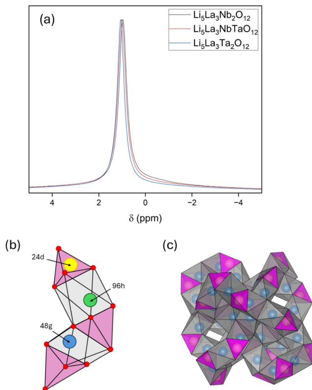
Fig. 10 (a) {}^7\text{Li} (14.1 T, 20 kHz MAS) MAS NMR spectra of powder \text{Li}_5\text{-La}_3\text{M}_2\text{O}_{12} ( M = \text{Nb, Ta, Nb/Ta} ). (b) Tetrahedral and octahedral frameworks of oxygen (represented as red spheres at the polyhedral corners), which host Li atoms at specific sites: yellow (24 d, tetrahedral), blue (48 g, octahedral), and green (96 h, off-centre octahedral). (c) Illustrates the 3D network of connected oxygen polyhedron accommodating Li atoms (yellow and blue spheres).
