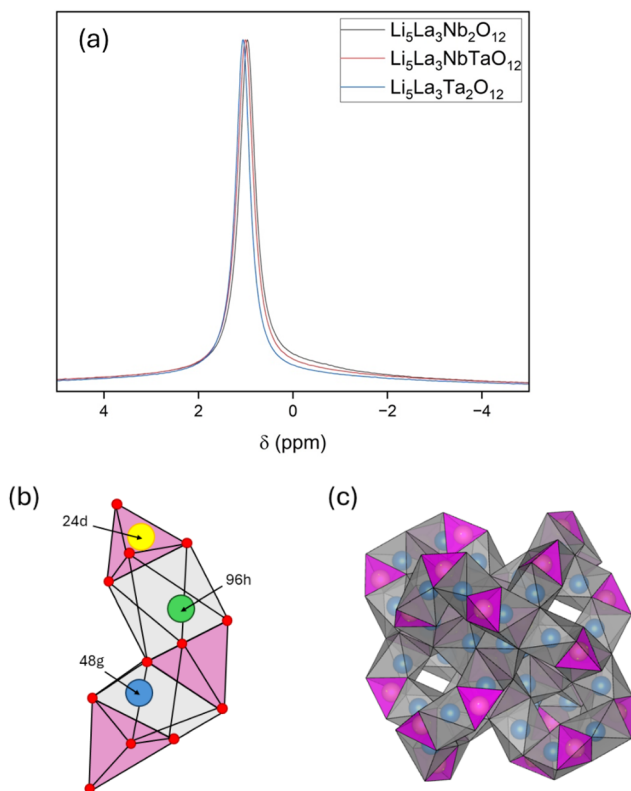
Fig. 10 (a) {}^7\text{Li} (14.1 T, 20 kHz MAS) MAS NMR spectra of powder \text{Li}_5\text{La}_3\text{M}_2\text{O}_{12} ( M = \text{Nb, Ta, Nb/Ta} ). (b) Tetrahedral and octahedral frameworks of oxygen (represented as red spheres at the polyhedral corners), which host Li atoms at specific sites: yellow (24 d, tetrahedral), blue (48 g, octahedral), and green (96 h, off-centre octahedral). (c) Illustrates the 3D network of connected oxygen polyhedron accommodating Li atoms (yellow and blue spheres).
