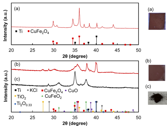
Fig. 2 XRD patterns and appearance of (a) the \text{CuFe}_2\text{O}_4 photocathode fabricated by the citric acid polymerization at 800\text{ }^\circ\text{C} , (b) the \text{CuFe}_2\text{O}_4\text{-CuO} photocathode fabricated by the hydrothermal synthesis at 120\text{ }^\circ\text{C} followed by the heat treatment at 650\text{ }^\circ\text{C} , and (c) the as-synthesized powder at 120\text{ }^\circ\text{C} . Reference PDF data of \text{CuFe}_2\text{O}_4 , \text{CuO} , \text{CuFeO}_2 , \text{Ti} , \text{TiO}_2 and \text{KCl} are also indicated.
