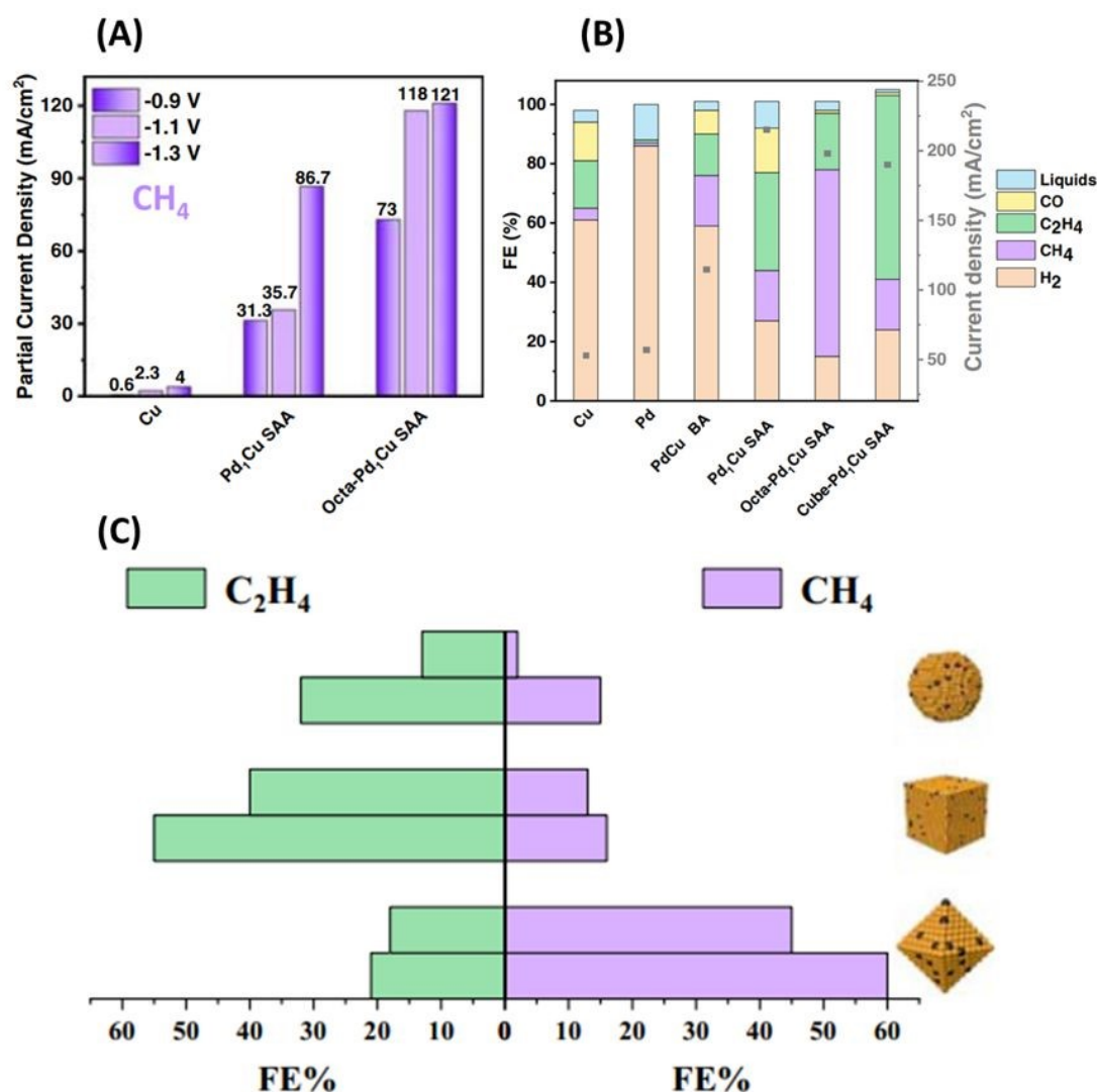
Figure 7: (A) Partial current density for CH_4 at different voltages for polycrystalline Cu, polycrystalline Pd 1 Cu configuration and shape-controlled Octa-Pd 1 Cu configuration. SAA stands for single-atom alloys. (B) Comparison of CO 2 reduction FE (%) and current densities of Pd 1 Cu configuration and analogues. The FE was obtained from amperometric i -t curves at -1.1 V vs RHE (in a CO 2 -saturated 0.5 M KHCO 3 solution) and quantifying the products over 30 min. (C) FE distribution of CH_4 and C_2H_4 obtained using Cu and shape controlled Pd 1 Cu materials. Reproduced from reference 106 with permission from Springer Nature, copyright 2023.
