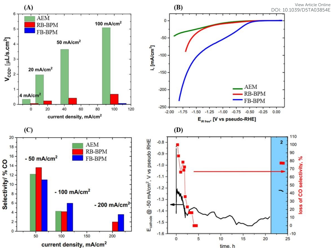
Figure 10: (A) Volume flows of CO 2 produced at the anode side of a CO 2 -electrolyzer cell with an Au-based cathode and an IrO 2 -TiO 2 anode catalyst using different membrane configurations. The anode gas composition was analyzed using mass spectrometry at various cell current densities in galvanostatic mode. Cells were operated at 40°C under ambient pressure. The cathode was fed with pure, humidified CO 2 and the anode with humidified Ar. (B) Cathode polarization curves of CO 2 - electrolysis cells with AEM (Fumasep AA30), RB-BPM (Fumatech FBM, 130 \mu\text{m} thickness), and FB-BPM (Fumatech FBM, 130 \mu\text{m} thickness) at 50 \text{mV s}^{-1} , 40 °C and ambient pressure. (C) CO selectivities obtained in galvanostatic experiments at various fixed current densities. (D) Chronoamperometric measurements at - 50 \text{mA cm}^{-2} (black line) and corresponding CO selectivity measured by online MS (red data) for the FB-BPM. The cathode was fed with 50/50 vol.% CO 2 /Ar, while the anode consisted of Pt/C catalyst fed with pure H 2 . Reproduced from reference 165 with permission from ECS, copyright 2019.
