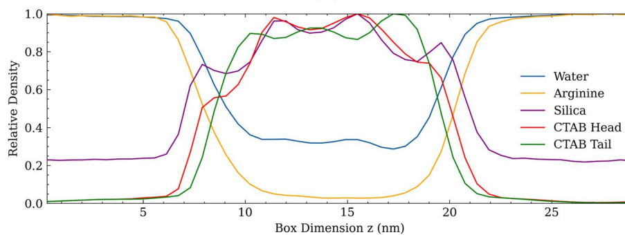
Fig. 7 Snapshots of the final configuration after 6 \mu s are shown for self-assembly simulations without additive (a) and with arginine ((b) and (c)) starting from a random configuration. CTAB headgroups are shown in red, tails in green, silica dimers in purple and arginine in orange. Water is hidden in all snapshots for clarity. In (d), the time averaged relative densities (calculated as \rho/\rho_{\text{max}} ) across the z axis for all species are shown. The black arrow in (b) points towards a single arginine case observed in the surfactant phase.
