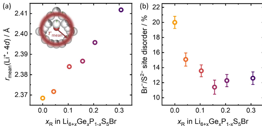
Fig. 4 Structural changes in Li + substructure of Li 6+x Ge x P 1-x S 5 Br. (a) The r_{\text{mean}} distance between the 4d site and the Li + increases, indicating a more spread-out Li + distribution. (b) The Br - /S 2- site disorder decreases with the onset of Ge(IV) incorporation and then remains approximately constant for increasing Ge(IV) contents.
