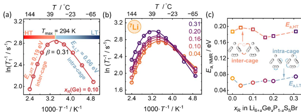
Fig. 6 Solid-state {}^7\text{Li} spin-lattice ( T_1 ) relaxometry for the substitution series of \text{Li}_{6+x}\text{Ge}_x\text{P}_{1-x}\text{S}_5\text{Br} . (a) Representative Arrhenius plot of {}^7\text{Li} T_1 -relaxation measurement for \text{Li}_{6.10}\text{Ge}_{0.10}\text{P}_{0.90}\text{S}_5\text{Br} and (b) for the substitution series of \text{Li}_{6+x}\text{Ge}_x\text{P}_{1-x}\text{S}_5\text{Br} . (c) Activation energies obtained from a modified BPP fit, corresponding to the high-temperature and low-temperature flank of the rate peaks.
