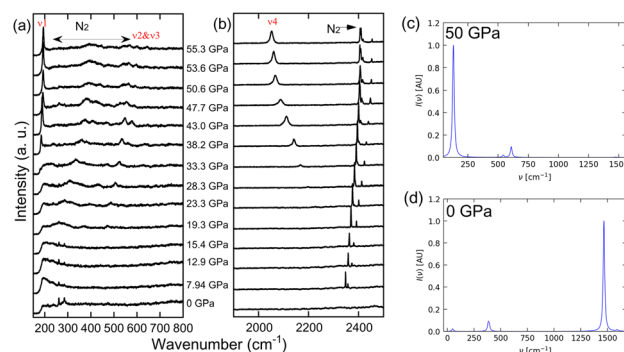
Fig. 5 Pressure dependence of the measured (AG#2) and calculated Raman spectra. Two wavenumber regions are separately shown in (a) and (b). Newly appeared peaks are represented with \nu_i ( i = 1\text{--}4 ). Wavenumber regions corresponding to the \text{N}_2 pressure medium are represented with horizontal arrows. Spiky peaks at low wavenumber regions at low pressures might be derived from the instruments or atmospheric species. Calculated Raman spectra of I4/mcm \text{PbN}_2 at 0 K (c) 50 GPa and (d) 0 GPa.
