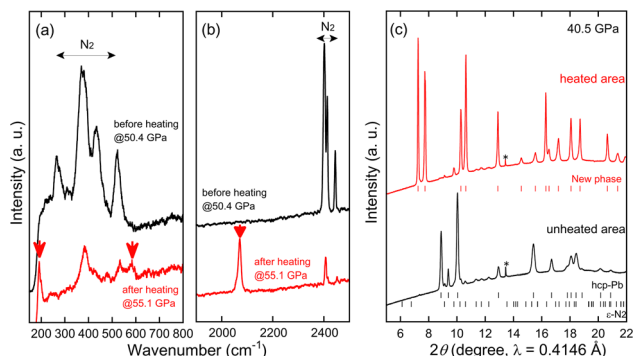
Fig. 1 Raman spectra and XRD profiles under high pressures. (a) and (b) shows the Raman spectra corresponding to the \text{Pb}-\text{N}_2 sample (AG#1) before and after laser heating at approximately 50 GPa. Two wavenumber regions were separately displayed. Intense peaks after laser-heating are marked with arrows. The horizontal arrows show the wavenumber region derived from solid molecular nitrogen. (c) High-pressure in situ X-ray diffraction profiles acquired from the heated and unheated areas. The diffraction peak positions of Pb, and \text{N}_2 are represented with ticks at the bottom of the profiles. The intense peak positions derived from the new phase that appeared after laser heating are also indicated with ticks. The peak marked with an asterisk might be derived from the device.
