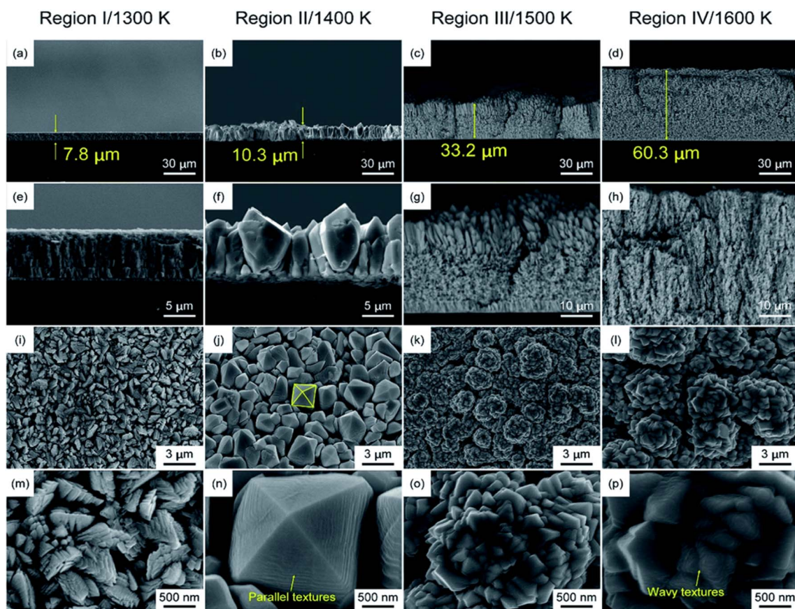
Fig. 4 SEM images of the cross-sections and surfaces of HfO_2 films in the four regions, obtained using the high-throughput growth process. (a), (e), (i), (m) region I at T = 1300 \text{ K} , (b), (f), (j), (n) region II at T = 1400 \text{ K} , (c), (g), (k), (o) region III at T = 1500 \text{ K} , (d), (h), (l), (p) region IV at T = 1600 \text{ K} , respectively. T represents deposition temperature, reused with permission from Royal Society of Chemistry. 342
