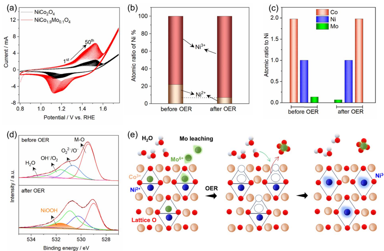
Fig. 4 (a) CV measurements of \text{NiCo}_2\text{O}_4 and \text{NiCo}_{1.9}\text{Mo}_{0.1}\text{O}_4 (50 cycles), (b) atomic ratios of \text{Ni}^{2+} and \text{Ni}^{3+} in \text{NiCo}_{1.9}\text{Mo}_{0.1}\text{O}_4 before and after the OER, (c) surface atomic concentration of Co, Ni and Mo, (d) O 1s XPS spectra in \text{NiCo}_{1.9}\text{Mo}_{0.1}\text{O}_4 before and after the OER, (e) schematic illustration of surface transformation in \text{NiCo}_{1.9}\text{Mo}_{0.1}\text{O}_4 showing \text{Mo}^{6+} leaching, cation vacancies, and \text{NiOOH} formation.
