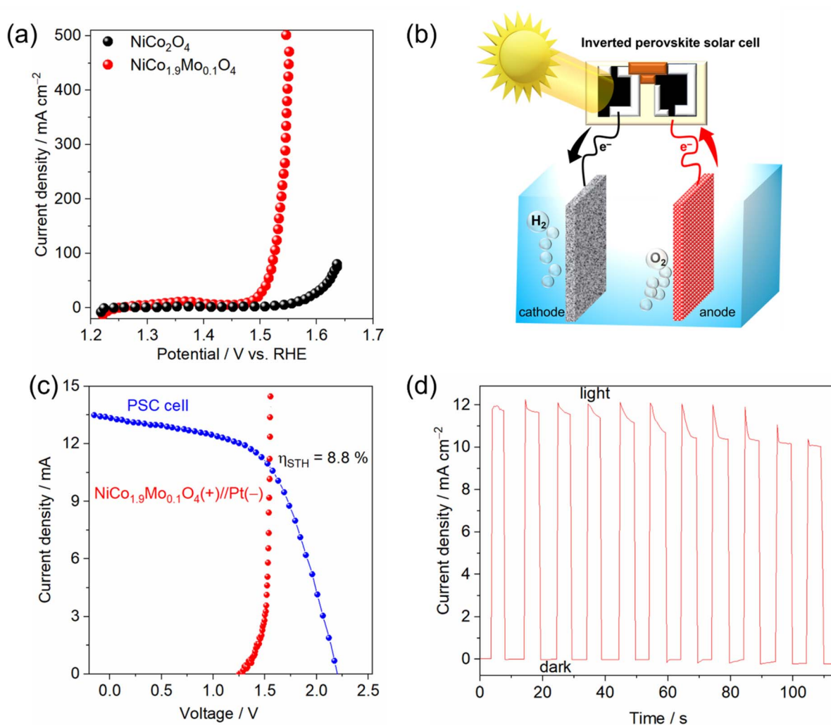
Fig. 5 (a) Polarization curves of \text{NiCo}_2\text{O}_4/\text{NF} and \text{NiCo}_{1.9}\text{Mo}_{0.1}\text{O}_4/\text{NF} , (b) schematic illustration of the PSC-driven water electrolysis, (c) current–voltage curves of the perovskite solar cell under 1 sun illumination ( \text{AM } 1.5 \text{ G} , 100 \text{ mW cm}^{-2} ) and /NF in a two-electrode cell configuration, (d) current–time plot of the water electrolysis system without external bias potential ( V = 0 ) under 1 sun illumination.
