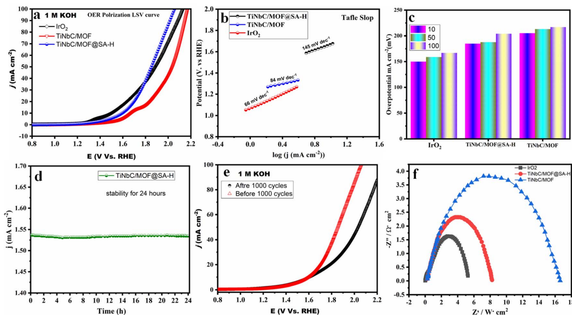
Fig. 7 (a) OER polarization LSV curves, (b) Tafel slope, (c) the overpotentials required for achieving \eta = 10, 50 and 100 mA cm -2 (mV), (d) stability curve for 24 h, (e) KOH LSV curve after and before 1000 cycles, and (f) Nyquist plots at 4.0 V RHE of IrO 2 , TiNbC/MOF and TiNbC/MOF@SA-H.
