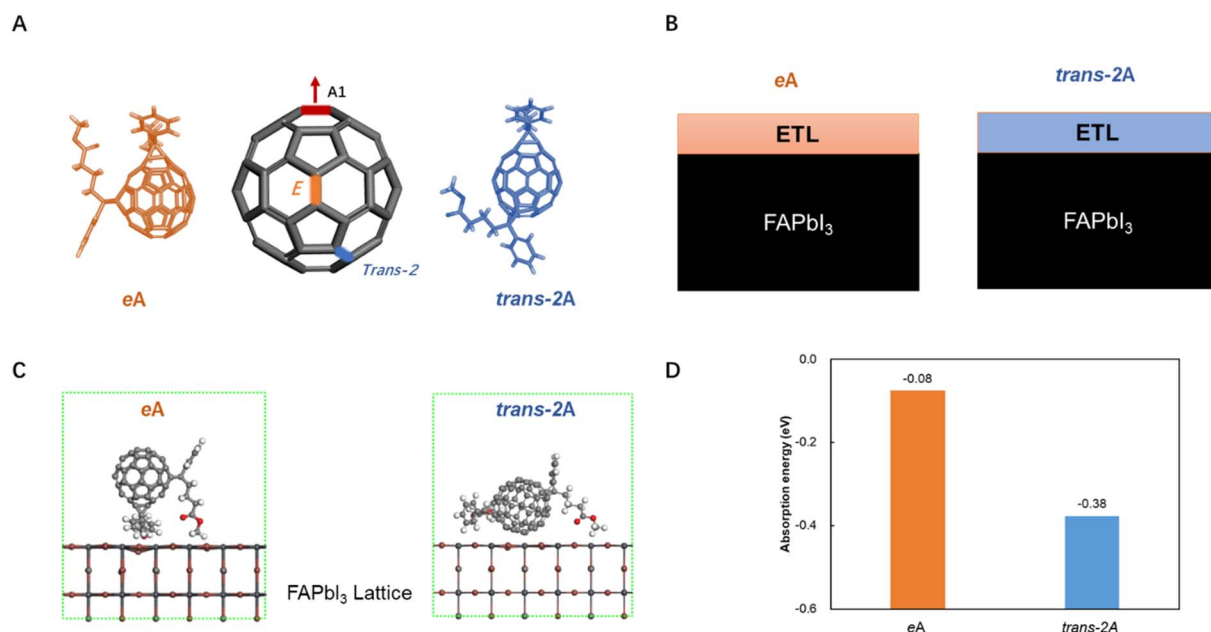
Fig. 2 Interfacial absorption energy between ETLs/perovskite interface. (A) Molecular structures of eA and trans -2A. (B) Schematic illustration of the bilayer structures of eA/ trans -2A ETLs on top of the perovskite, respectively. (C) Bonding between the FAPbI 3 (100) surfaces and trans -2A or eA. (D) Absorption energy of trans -2A/perovskite and eA/perovskite interface. The plane wave basis expansion had an energy cutoff of 400 eV, with partial occupancies handled by Gaussian smearing (0.2 eV width). Gamma point sampling was used for surface structure optimization, with convergence thresholds set at 10^{-4} eV for energy and 0.05 eV Å -1 for force. The bulk structure of FAPbI 3 was optimized with a 4 \times 4 \times 4 k -point, and the FAPbI 3 (100) surface contained 36 Pb, 36 C, and 108 I atoms.
