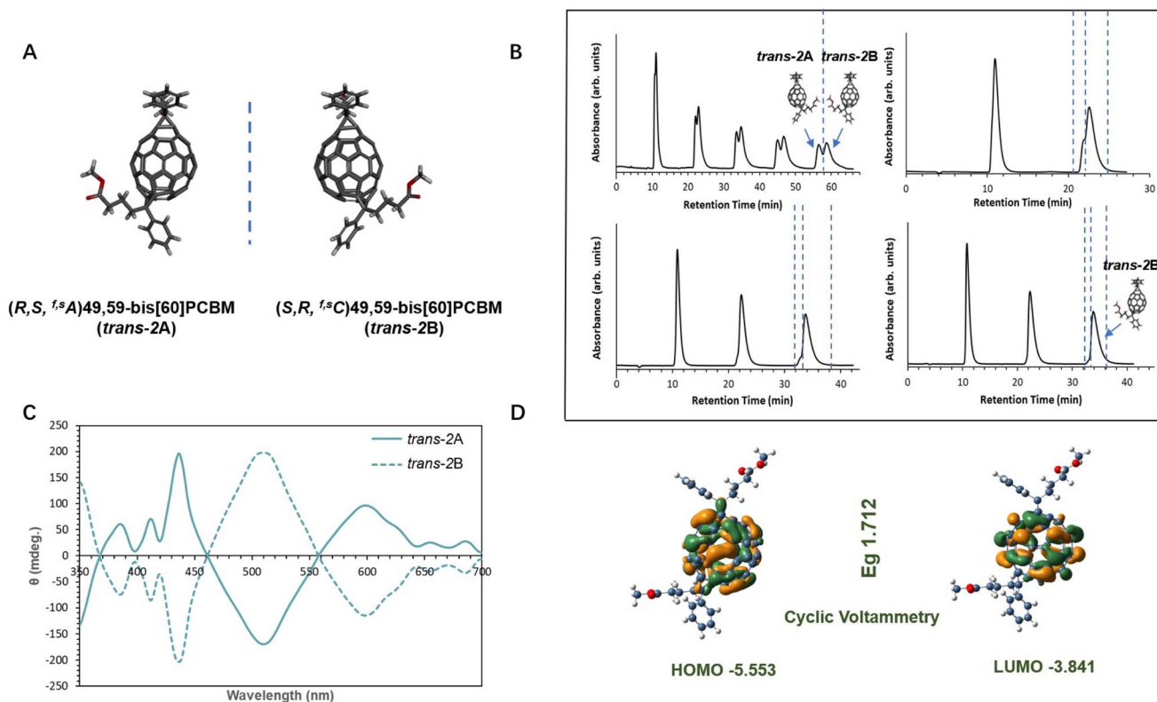
Fig. 1 Isolation and characterization of ( R,S , f s A )49,59-bis[60]PCBM ( trans-2A ) and ( S,R , f s C )49,59-bis[60]PCBM ( trans-2B ). (A) Molecular structures of each enantiomer. (B) Complete HPLC purification process for trans-2B , achieving purity exceeding 99% through peak-recycling HPLC. (C) Circular dichroism spectra of the enantiomers in toluene ( \sim 0.2 mg mL -1 ). (D) HOMO, LUMO, and energy gap of the enantiomers, along with molecular geometries determined using DFT at the B3LYP/6-311G (2df,2pd) level of theory.
