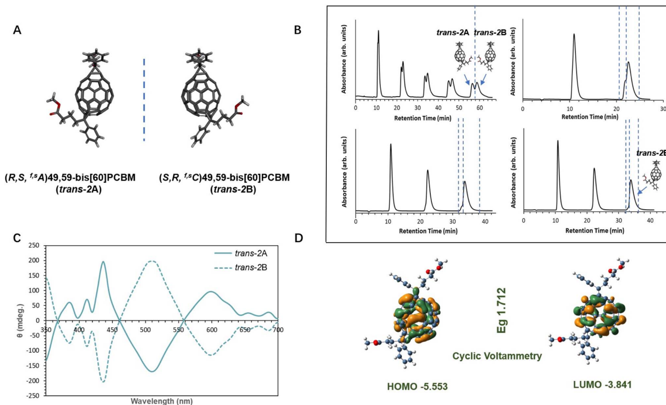
Fig. 1 Isolation and characterization of ( R , S , f s , A )49,59-bis[60]PCBM ( trans -2A) and ( S , R , f s , C )49,59-bis[60]PCBM ( trans -2B). (A) Molecular structures of each enantiomer. (B) Complete HPLC purification process for trans -2B, achieving purity exceeding 99% through peak-recycling HPLC. (C) Circular dichroism spectra of the enantiomers in toluene (~0.2 mg mL -1 ). (D) HOMO, LUMO, and energy gap of the enantiomers, along with molecular geometries determined using DFT at the B3LYP/6-311G (2df,2pd) level of theory.
