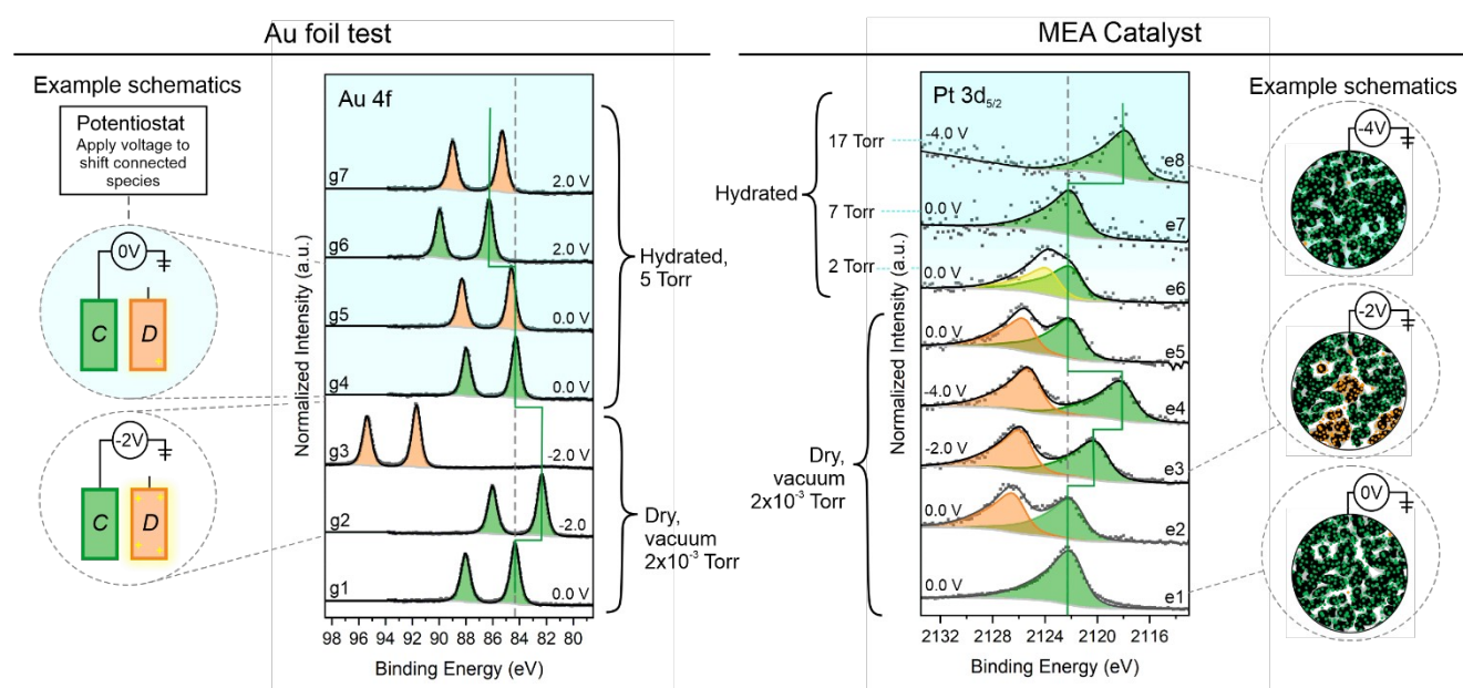
Figure 4: Particle connectivity trial as a function of potential and condition. Left: Au 4f spectra for an electrically connected (C) and disconnected (D) Au foil. Right: Pt 3d 5/2 XPS results for trials on a Pt-based MEA. Example schematics of the electrical setup are to the side of the spectral regions for some conditions.
