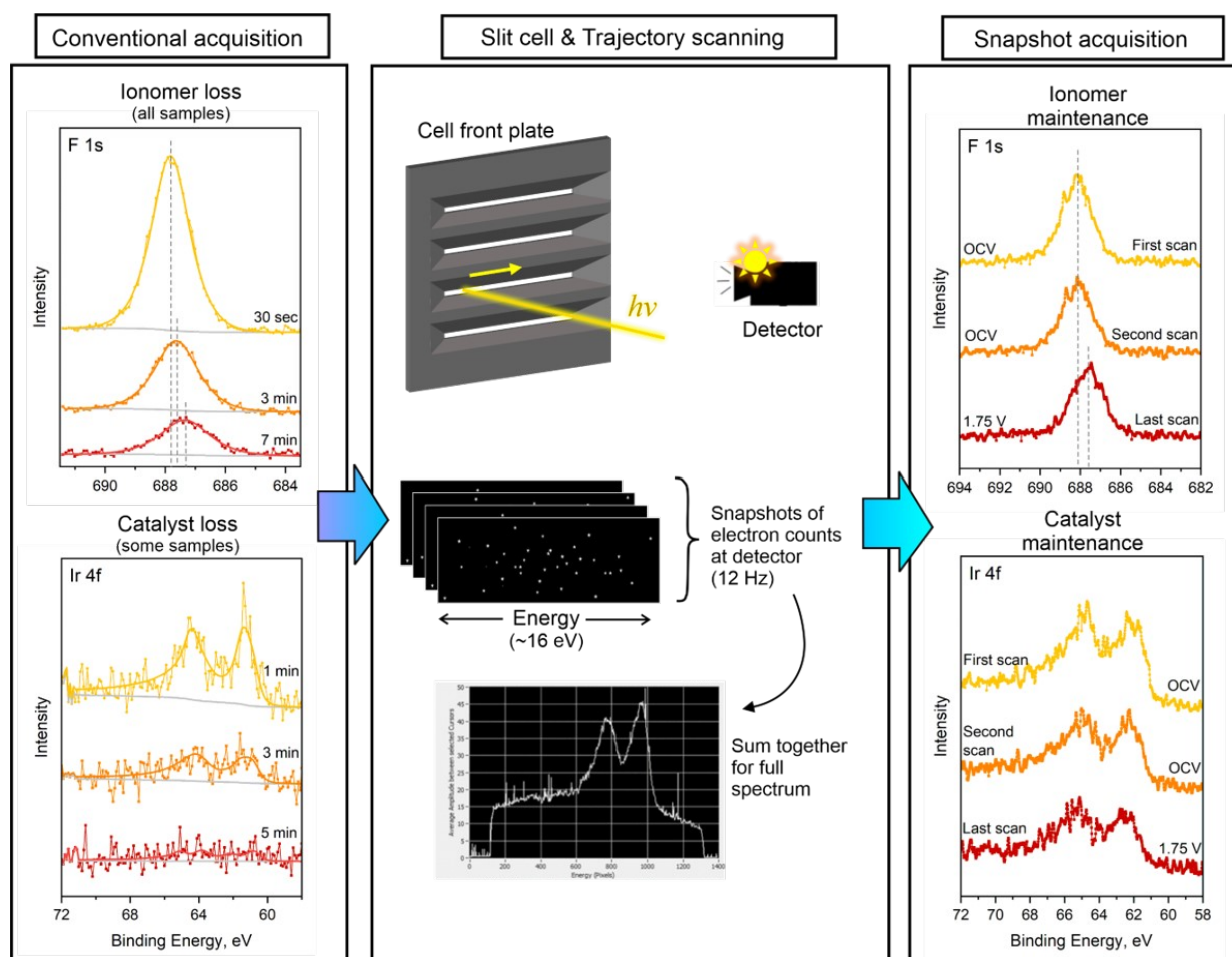
Figure 5: Beam effects and mitigation via trajectory scanning and snapshot collection mode. Left hand panel: conventional data acquisition leads to loss and a change in the electrode signal. Center: the cell #2 slit design keeps the sample flat and allows for use of trajectory scanning, while snapshot acquisition mode collects low-resolution spectra at a rate of 12 Hz, which are summed for higher quality spectra. Right panel: resulting stable signal from electrode components.
