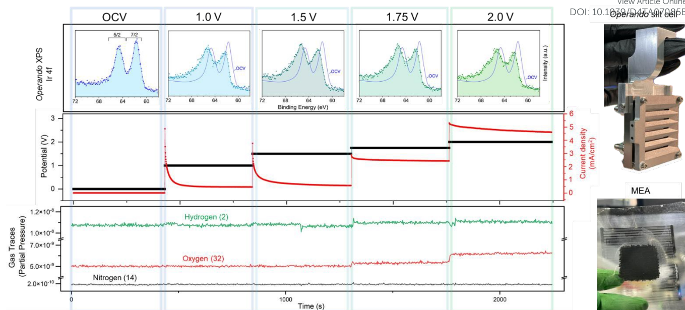
Figure 2: (Left) Data from the working 2-electrode cell of a TKK MEA (0.4 mg/cm 2 catalyst loading) with increasing anodic conditions (OCV – 2.0 V) from left to right. Top row is the operando AP-XPS Ir 4f spectra for 5 polarization conditions, taken in standard collection mode at different locations on the sample freshly exposed to the X-ray. The OCV data envelope (blue) is included in the other 4 anodic plots for comparison. The middle panel shows the corresponding data for the chronoamperometry applied voltage and measured current density. The bottom panel shows the partial pressure gas traces from the RGA. (Right) Images of the operando slit cell (cell #2) and a standard MEA.
