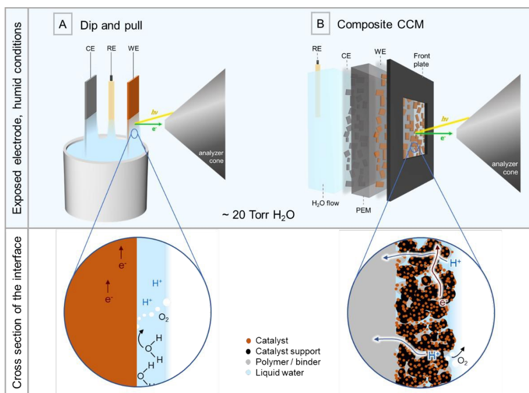
Figure 1: Schematic comparing two exposed-electrode experimental set-ups for operando electrochemical AP-XPS. A) A ‘dip and pull’ 3-electrode system for model electrocatalyst studies in liquid electrolyte. B) The operando cell with an opening for access to the working electrode on a composite catalyst-coated membrane (CCM). This may be used in a 2 or 3 electrode configuration.
