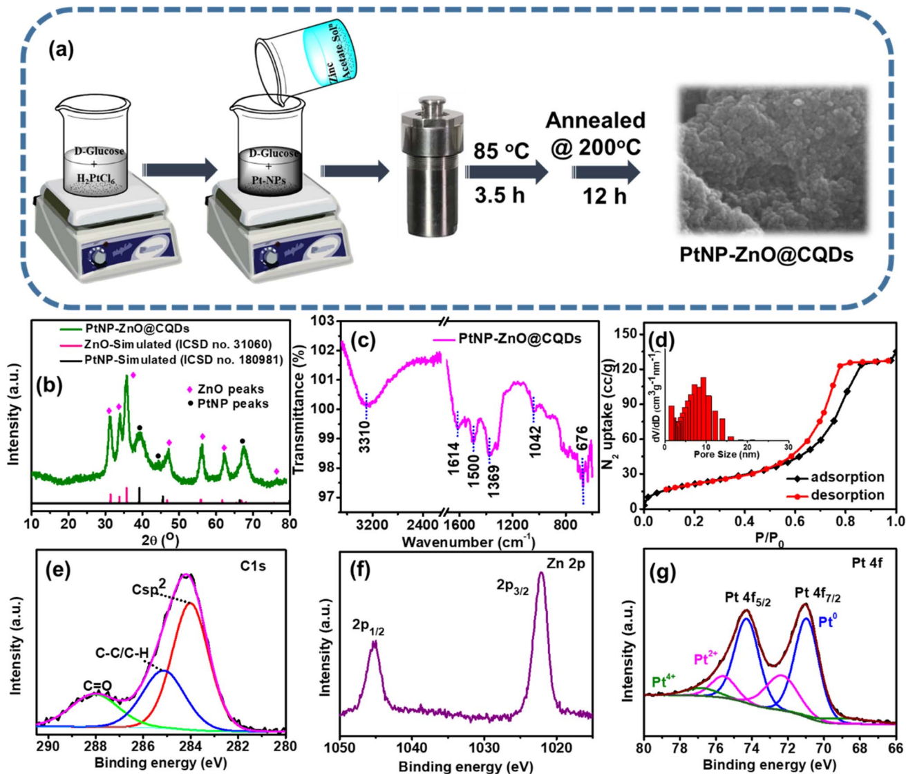
Fig. 1 (a) Schematic diagram of the synthesis of PtNP-ZnO@CQDs. (b) X-ray diffraction pattern of PtNP-ZnO@CQDs compared with simulated ZnO and PtNP patterns. (c) FT-IR of PtNP-ZnO@CQDs. (d) \text{N}_2 -isotherm of PtNP-ZnO@CQDs. The pore size distribution plot is given in the inset. Core level XPS spectra of (e) C 1s, (f) Zn 2p, and (g) Pt 4f.
