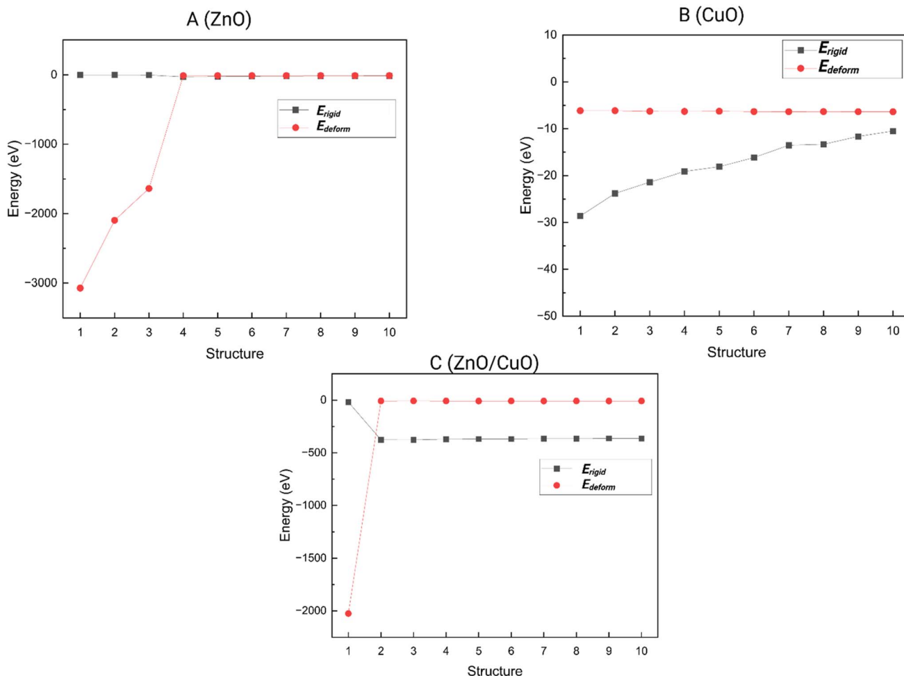
Fig. 10 Deformation energy ( E_{deform} ) and rigid adsorption energy ( E_{rigid} ) for ZnO–CBC; CuO–CBC; and (ZnO + CuO)–CBC adsorption simulations with 10 different configurational structures ((A) ZnO–CBC; (B) CuO–CBC; (C) [ZnO + CuO]–CBC).
