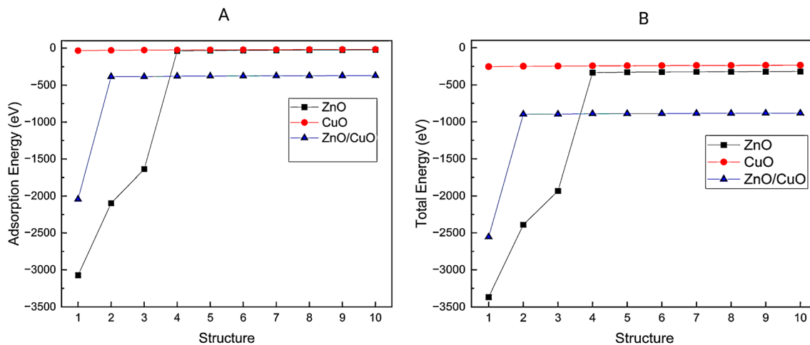
Fig. 9 Adsorption energy ( E_{ads} ) and total energy ( E_{total} ) for ZnO–CBC, CuO–CBC and [ZnO + CuO]–CBC complexes for 10 different configurational structures ((A) adsorption energy and (B) total energy).
