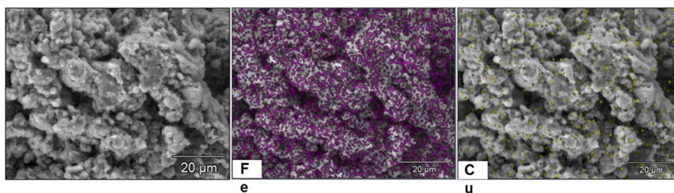
Fig. 16 SEM, Fe, and Cu elemental mapping image of \text{Fe}_3\text{O}_4@KNPs\text{-Cu(II)} after five cycles of catalytic tests.
