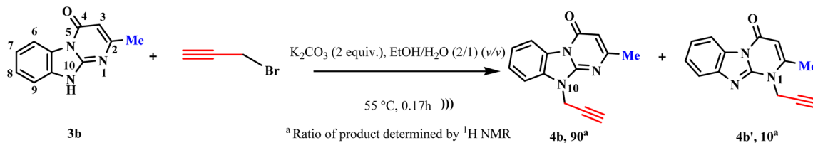
Scheme 4 Regiosomeric mixture of 4b and 4b' .
