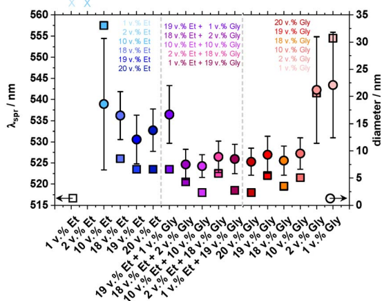
Fig. 2 \lambda_{\text{SPR}} values retrieved from UV-vis characterization (□, left-hand side axis) and NP diameter (○, right-hand side axis) retrieved from STEM analysis as a function of different alcohol contents and mixtures, as indicated. The source of reducing agent was ethanol only in various contents, [ethanol + glycerol] in various ratios, and glycerol only in various contents, as indicated. X indicates samples for which the plasmon resonance is not well pronounced: 1 and 2 v% ethanol. Et: ethanol; Gly: glycerol. See Fig. S2† for UV-vis spectra and Fig. S3† for further correlation between \lambda_{\text{SPR}} and diameter. In all cases 0.5 mM HAuCl 4 and 2 mM NaOH were used.
