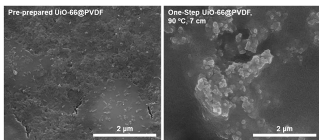
Fig. 2 SEM images obtained for the UiO@PVDF membranes prepared by dispersing pre-synthesized UiO-66 in a PVDF solution (left) and using the one-step method (right). Note how the one-step method ensures MOF particles are present in the membrane's surface.
