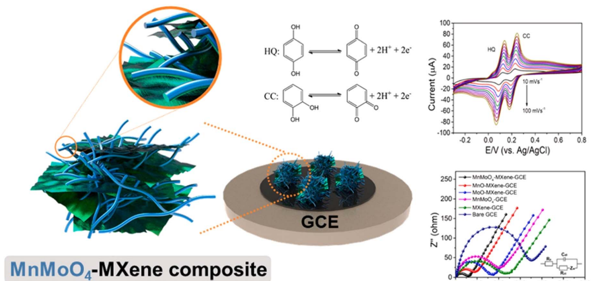
Fig. 14 Modification of the surface of GCE using the \text{MnMoO}_4 -MXene nanocomposite material for the detection of hydroquinone and catechol. 145 Copyright, adopted from Elsevier.
