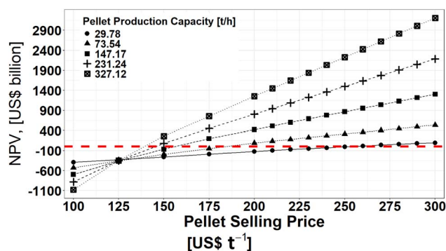
Fig. 8 Net present value for 30–330 t per h Pellet Plant A at the baseline (10%) discount rate, a camelina straw feedstock cost of US$48.84 per t, for a range of pellet prices, and 100% capacity utilization (assuming zero revenue from selling mushrooms).
