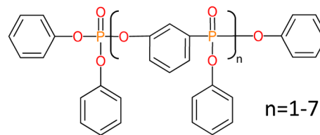
Fig. 1 Chemical structure of RDP.
