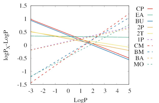
Fig. 4 Extraction efficiencies from water of the individual biobased solvents relative to 1-octanol (log P_x - \log P ). The lines show the linear regressions from Fig. 3. Positive values mean that the solvent exhibits a higher extraction efficiency than 1-octanol. The selected green solvents are abbreviated as cyclopentanol (CP), ethyl acetate (EA), 1-butanol (BU), 2-pentanol (2P), 2-methyl tetrahydrofuran (2T), 1-pentanol (1P), cyclopentyl methyl ether (CM), butyl methyl ether (BM), butyl acetate (BA), and methyl oleate (MO). Some solvents show significantly higher extraction yields than 1-octanol: cyclopentanol, and 1-butanol for hydrophilic solutes (log P < 0.5), as well as cyclopentyl methyl ether and butyl methyl ether for hydrophobic solutes (log P > 2.6). For log P values in the range between 0.5 and 2.6, ethyl acetate and 1-pentanol are the most efficient extraction solvents from water.
