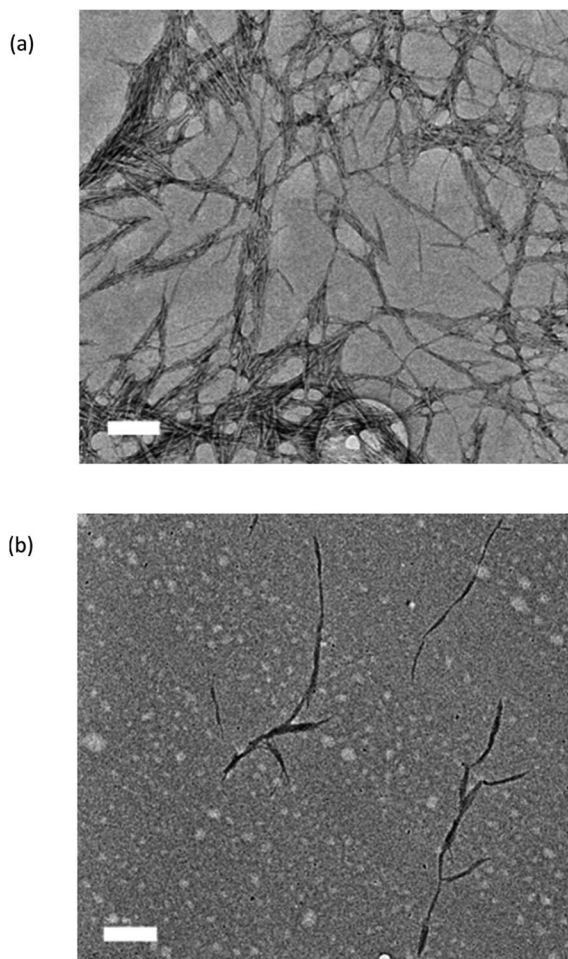
Fig. 3 TEM images of (a) wet NCC (W-NCC) and (b) spray-dried NCC (SD-NCC) at 100 00× magnification.
