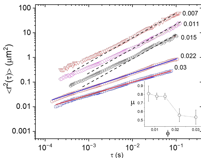
Fig. 3. The log-log plot of mean-square-displacement, \langle r^2(\tau) \rangle vs. lag time of nanorods in BSM solutions. The graphs have been shifted vertically for clarity. The different volume fractions were as indicated next to the data. The dashed lines for the three lowest concentrations have a slope of 1 and showed the transition from subdiffusive motion at short time to normal diffusion at long time. There was no subdiffusion observed for the two higher concentration solutions within the experimental time range. (inset) The short-time subdiffusive exponent for different concentrations.
