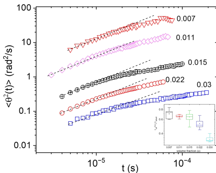
Fig. 4. The mean-square-angular displacement (MSAD) vs. lag time extracted from the rotational part of the correlation function. The graphs have been shifted vertically for clarity. The dashed lines have slope of 1. The corresponding volume fractions are indicated. (inset) The relative slow down of short-time rotational diffusion coefficient compared to buffer for different concentration.
