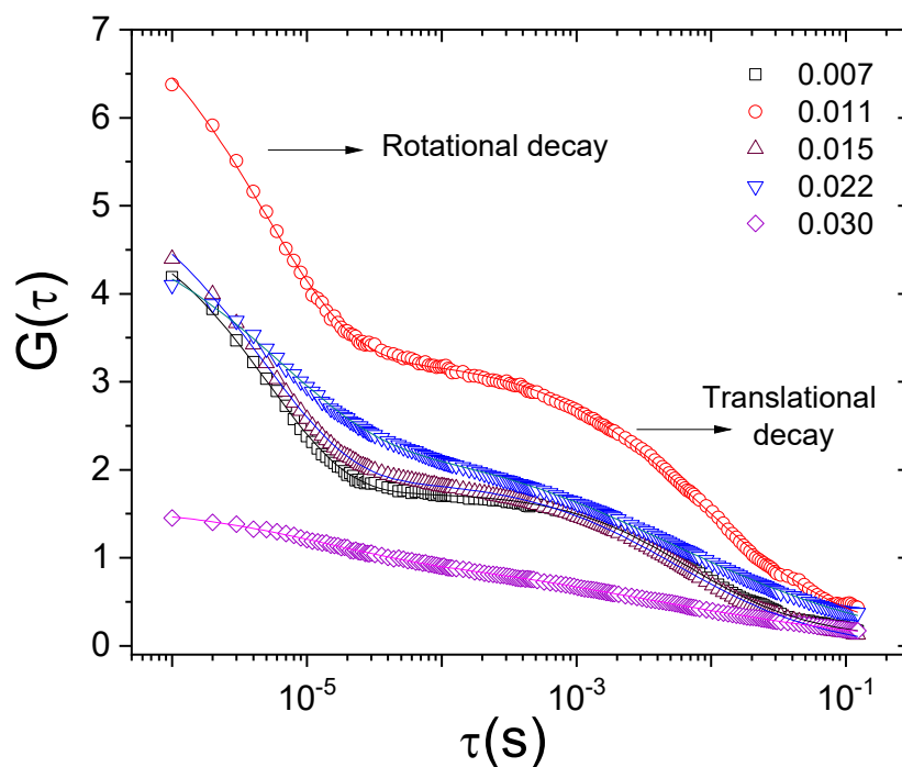
Fig. 1. Representative autocorrelation functions (ACFs) of gold nanorods with core dimensions of 10 nm × 38 nm, dispersed in bovine submaxillary mucin (BSM) solutions. (Graphs are vertically shifted for clarity) The nanorods were surface-functionalized with 3 kDa PEG–carboxyl ligands. The volume fractions ( \phi ) of mucin are indicated. The ACFs exhibit two-step decay: the fast decay corresponds to rotational motion, while the slower decay reflects translational diffusion. Solid lines represent fits using the model described in the main text, yielding the mean residence time within the confocal volume ( \langle\tau_c\rangle ), the rotational correlation time ( \langle\tau_r\rangle ), and the associated anomalous diffusion exponents \alpha and \beta .
