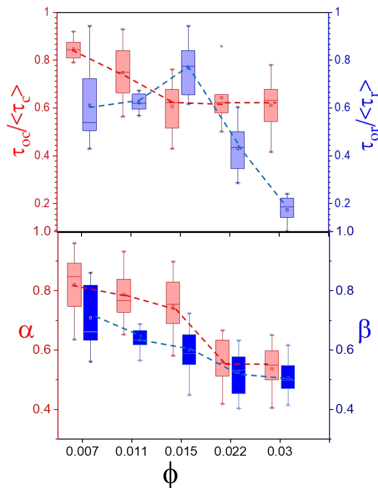
Fig. 2. (Top) Box-and-whisker plots showing the mean residence times for translational diffusion (left axis) and rotational correlation times (right axis) of nanorods in BSM solutions. All values are normalized to their respective measurements in buffer ( \tau_{oc} \approx 4.9 ms, \tau_{or} \approx 4.7 \mu s). Dashed lines are included to guide the eye. (Bottom) The anomalous exponents, rather than the absolute timescales of motion, associated with translation ( \alpha , left) and rotation ( \beta , right). A strong subdiffusive behavior emerges at higher concentrations. At the highest volume fractions, translational exponents approach \alpha \approx 0.5 , consistent with Rouse-like dynamics.
