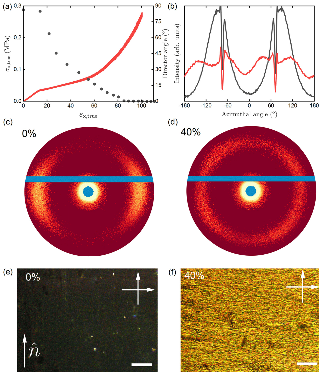
Fig. 6 (a) Stress–strain response of the 1/8\times LCE at a strain rate of 0.1\text{ min}^{-1} plotted as a function of true-stress ( \sigma_{x,\text{true}} ) and true-strain ( \epsilon_{x,\text{true}} ) (red line) and director angle as a function of strain as determined via simultaneous observations with crossed polarizers (black circles). (b) X-ray scattering profile as a function of azimuthal angle for the 1/8\times sample under \epsilon_{x,\text{true}} = 0\% (black) and \epsilon_{x,\text{true}} = 40\% (strain). (c) and (d) 2D X-ray scattering image of the 1/8\times sample at \epsilon_{x,\text{true}} = 0\% and \epsilon_{x,\text{true}} = 40\% , respectively. (e) and (f) Polarised optical microscopy images of the 1/8\times sample at \epsilon_{x,\text{true}} = 0\% and \epsilon_{x,\text{true}} = 40\% , respectively. The arrows in (e) and (f) show the direction of the polariser and analyser, \hat{n} defines the orientation of the director in the unstrained sample. Scale bar = 75\text{ }\mu\text{m} .
