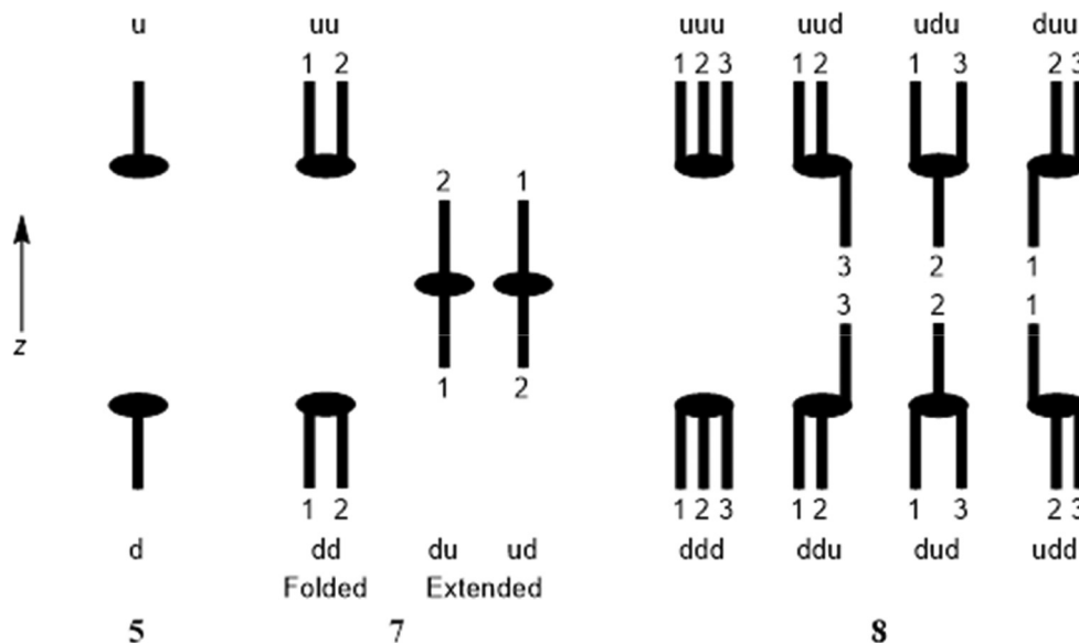
Fig. 9 Schematic representation of the general forms of 5, 7, and 8; the ovals represent the head-groups, the sticks represent numbered alkyl chains that may point independently either down (d) or up (u), and the respective pairs of down/up forms are related by a horizontal 180^\circ molecular rotation. The vertical sticks represent a wide range of possible conformers for each alkyl chain.
