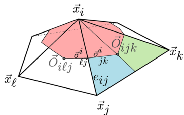
Fig. 16 Schematic of a vertex and its neighbors. The vertex i has neighbors, l, j, k, \dots , which are connected by edges e_{ij}, \dots , where we explicitly show e_{ij} . Each triangle has a circumcenter O , and the area is assigned to each of the 3 vertices, which is shown for triangle ijk (red, green, and blue section). The total area assigned to i is shown in red across the entire cap, and the dual edge \sigma^i across e_{ij} are shown \sigma^i_{jk} and \sigma^i_{jl} . The curvature of vertex i is essentially computed on the red area, for example, the normal of the vertex N(i) is the average of the local normal for every point in the red surface.
