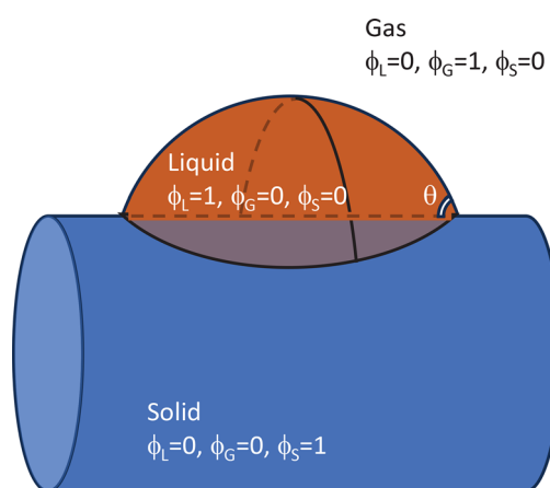
Fig. 1 Basic concepts in this study. The 3D liquid-droplet shape is represented by \phi_L(\mathbf{r}) = \phi(\mathbf{r}) , the primary focus of the calculation. The solid profile is fixed at a pre-specified \phi_S(\mathbf{r}) and the gas profile is deduced from the relation \phi_G(\mathbf{r}) = 1 - \phi_L(\mathbf{r}) - \phi_S(\mathbf{r}) . Far from the interfaces, each of these fields approaches the idealized bulk values, as illustrated in the sketch. A three-component phase-field model is used for \phi , \phi_S and \phi_G .
