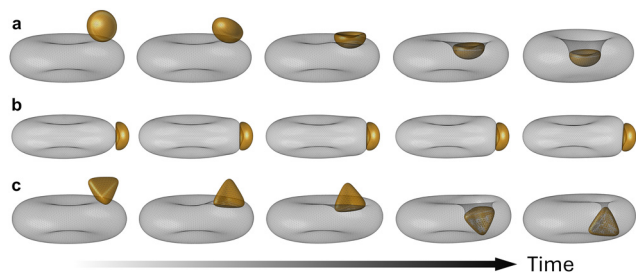
Fig. 8 Biconcave vesicle interaction with bowl-shaped and tetrahedral particles. (a) Bowl-shaped particle ( u_{\text{mod}} = 6.0 ) initially contacting the vesicle with its rim sinking into the concavity. (b) Bowl-shaped particle ( u_{\text{mod}} = 10.0 ) minimally adheres to the vesicle waist. (c) Tetrahedral particle ( u_{\text{mod}} = 10.0 ) rolls into the vesicle concavity. Images progress from left to right over simulation time.
