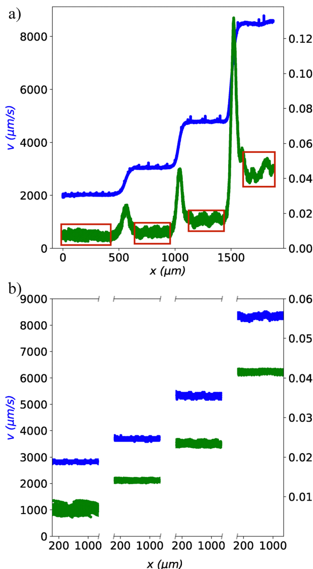
Fig. 3 Representative examples of velocity v and deformability D as a function of x in the flow direction for the linear and stacked arrangement of constrictions. For each constriction geometry, a single microscopy image captures all four constrictions of each device. In the linear arrangement, the widest constriction starts at x \lesssim 550 \mu\text{m} and the narrowest constriction ends at x \gtrsim 1700 \mu\text{m} . The red boxes indicate the region of measurement within each constriction. In the stacked arrangement, all constrictions extend the entire width of a microscopy image. Break points along the x axis indicate separate sections. For (a), data is obtained for droplets with \chi = 1.39 \times 10^{-2} . For (b), data is obtained for \chi = 1 \times 10^{-3} .
