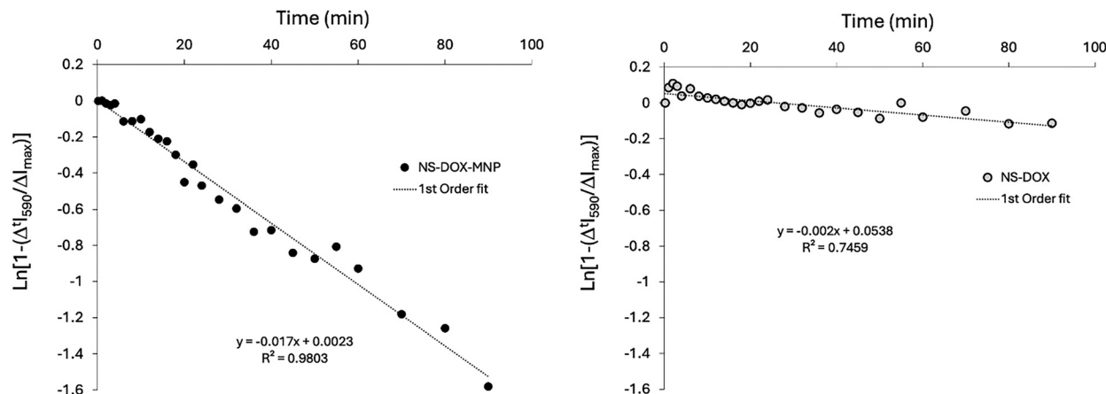
Fig. 7 1st order kinetic plots for NS-DOX-MNP sample (left) and the NS-DOX sample (right). \Delta I_{590} is the change in fluorescent intensity at 590 nm = (I_{590} - I_{800}) - (I_{590}^0 - I_{800}^0) , where I_{590} and I_{800} are the fluorescent intensity for time t at 590 nm and 800 nm respectively and I_{590}^0 and I_{800}^0 are the fluorescent intensity for time = 0 at 590 nm and 800 nm respectively.
