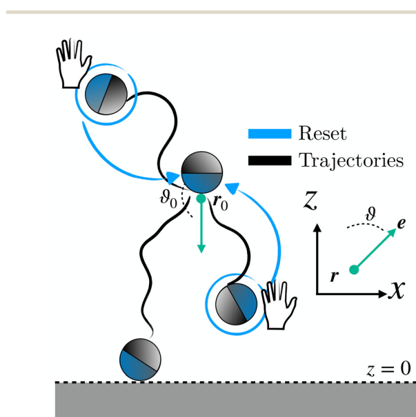
Fig. 1 Schematic of the motion of an ABP under stochastic resetting to its initial position \mathbf{r}_0 and orientation \vartheta_0 near an absorbing boundary at z = 0 . The green dot and arrow represent the resetting position and orientation, respectively. The inset depicts the agent's position \mathbf{r} and orientation \vartheta .
