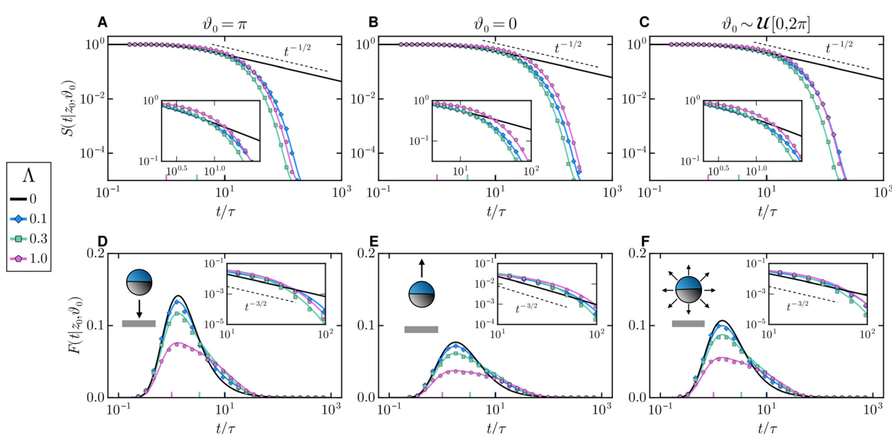
Fig. 6 Survival probability (A)–(C) and FPT probability density (D)–(F) as a function of time t for three different initial angles \vartheta_0 : the particle is initially (A) facing the wall, (B) facing against the wall, and (C) randomly oriented with an angle drawn from a uniform distribution \mathcal{U}[0, 2\pi] . Here, the initial position is z_0/a = 3 and the Péclet number is \text{Pe} = 0.4 . Solid lines and symbols denote theory and simulations for different resetting rates, respectively. The black lines represent the active case in the absence of resetting. The insets show a zoomed-in region of the plot containing them. The colored vertical lines represent the typical resetting times 1/\Lambda .
