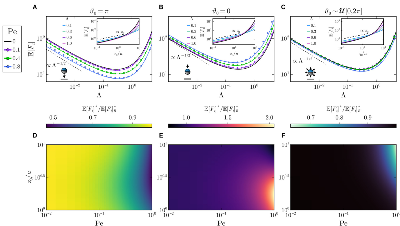
Fig. 2 (A)–(C) Mean first-passage time \mathbb{E}[F_i] for three different initial angles \vartheta_0 as a function of the resetting rate \Lambda (with z_0/a = 3 ) for different Péclet numbers Pe. Insets show the MFPT as a function of the initial distance z_0 for several \Lambda and Pe = 0.5. (D)–(F) Ratio of the mean first-passage times of an active and passive Brownian particle at the optimal resetting rate \mathbb{E}[F_i]^* / \mathbb{E}[F_i]_B^* as a function of Pe and z_0 . Columns show results for particles (A) and (D) initially facing the wall, (B) and (E) initially facing against the wall, and (C) and (F) with initial angles drawn from a uniform distribution \mathcal{U}[0, 2\pi] . Solid lines and markers denote theory and simulations, respectively. The black lines in (A)–(C) correspond to the passive case with resetting rate \Lambda_B = 1 .
