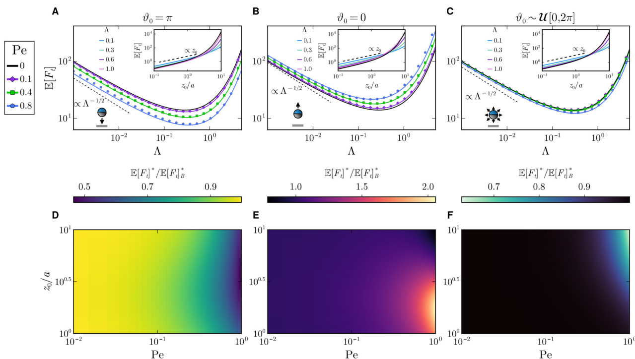
Fig. 2 (A)–(C) Mean first-passage time \mathbb{E}[F_i] for three different initial angles \vartheta_0 as a function of the resetting rate \Lambda (with z_0/a = 3 ) for different Péclet numbers \text{Pe} . Insets show the MFPT as a function of the initial distance z_0 for several \Lambda and \text{Pe} = 0.5 . (D)–(F) Ratio of the mean first-passage times of an active and passive Brownian particle at the optimal resetting rate \mathbb{E}[F_i]^* / \mathbb{E}[F_i]_B^* as a function of \text{Pe} and z_0 . Columns show results for particles (A) and (D) initially facing the wall, (B) and (E) initially facing against the wall, and (C) and (F) with initial angles drawn from a uniform distribution \mathcal{U}[0, 2\pi] . Solid lines and markers denote theory and simulations, respectively. The black lines in (A)–(C) correspond to the passive case with resetting rate \Lambda_B = 1 .
