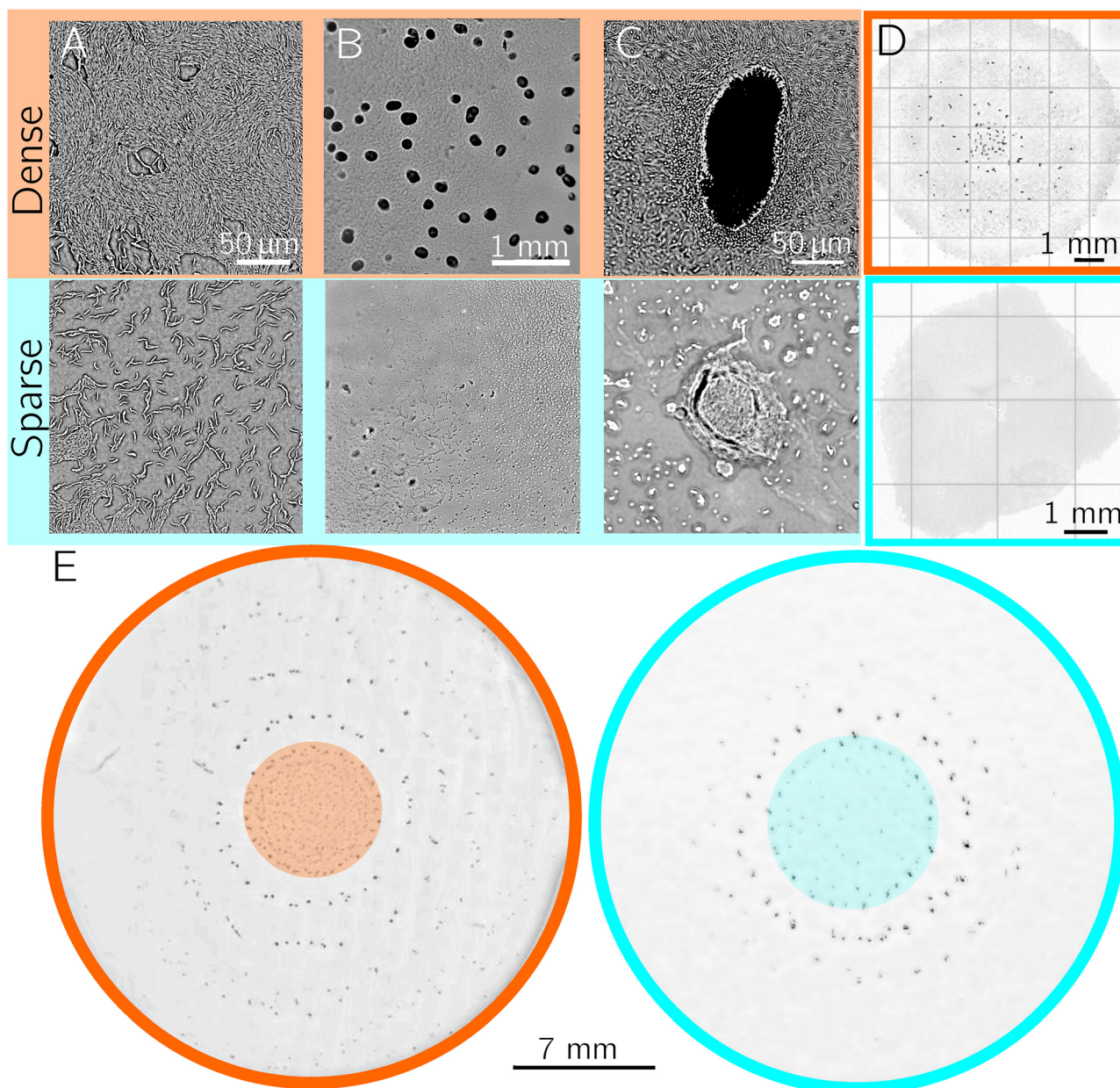
Fig. 5 Fruiting body formation (A) dense and sparse populations on TPM agar plates at the initial time point observed at 63× objective magnification. (B) Fruiting body formation at 4× objective magnification after 90 hours. (C) Close-up of a fruiting body at 63× objective magnification. (D) Comparison of the colony spread and fruiting body formation at 90 hours depending on the initial population density. The images result from the merging of adjacent pictures at 4× objective magnification. (E) Concentric pattern of fruiting bodies after one week of incubation. The fruiting bodies of dense and sparse populations are highlighted in black. The initial inoculation site of each population is at the center of the first ring, highlighted in color. The fruiting bodies are shown against a light background.
