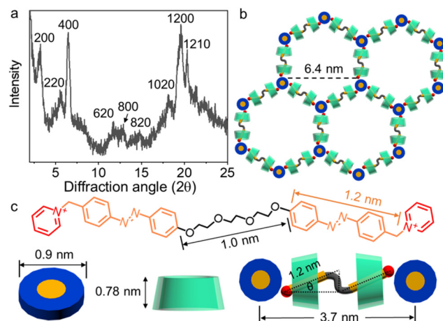
Fig. 1 (a) XRD pattern of the ISF xerogel, (b) corresponding simulated structure showing side spacing in ab plane, and (c) analysis of the framework structure in reference to the sizes of the AlMo 6 3- and CPR 2+ components.
