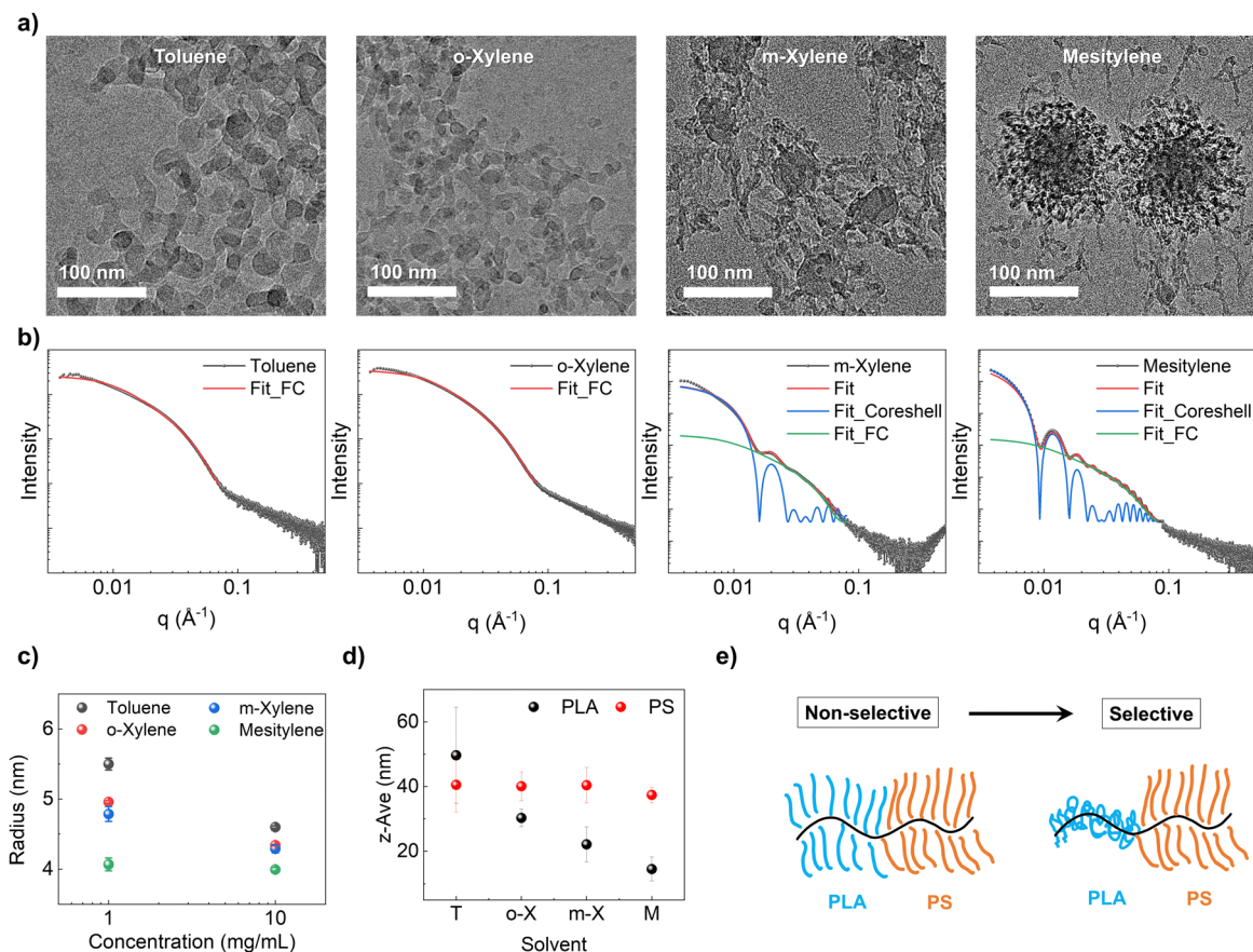
Fig. 4 (a) Cryo-TEM images of the BBCP in four different solvents (toluene, o -xylene, m -xylene, and mesitylene) at a concentration of 10 \text{ mg mL}^{-1} . (b) SAXS fitting curves of 10 \text{ mg mL}^{-1} solutions (black dots). For toluene and o -xylene, the flexible cylinder (FC) model was used for fitting (red curve). For m -xylene and mesitylene, a hybrid model comprising the core-shell model (blue curve) and flexible cylinder model (green curve) was employed for fitting. The red curves represent the overall fitting curve. (c) Fitted BBCP radius in different solvents (toluene: black, o -xylene: red, m -xylene: blue, and mesitylene: green) at solution concentrations of 1 and 10 \text{ mg mL}^{-1} . (d) The measured z -average size of PLA ( N_{\text{bb}} = 200 and N_{\text{sc}} = 60 , shown in black) and PS ( N_{\text{bb}} = 200 and N_{\text{sc}} = 45 , shown in red) homo bottlebrush polymers with different solvents in DLS experiments. (e) Schematic depicting the conformation of BBCPs in each solvent.
