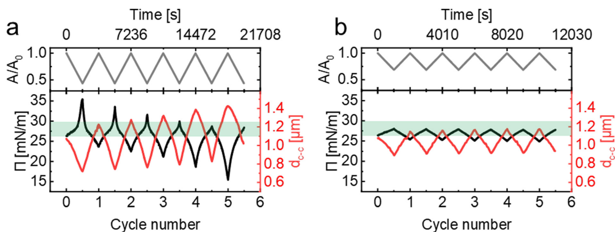
Fig. 5 Repeated compression/expansion cycles (each at 3 \text{ mm min}^{-1} ). Surface pressure \Pi and interparticle distance d_{c-c} as a function of cycle number and the normalized area A/A_0 as a function of time as a reference are shown. (a) Cycles compressed beyond region II and (b) with adjusted parameters to not exceed region II are presented. The green-colored area marks region II.
