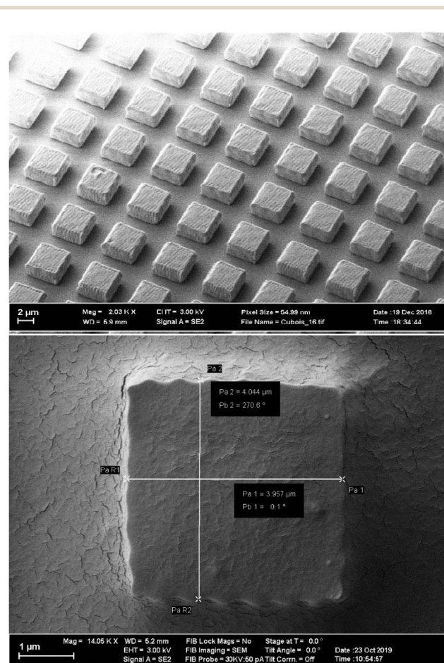
Fig. 1 Electron micrographs of squares written on a substrate after developing. The upper image serves as an overview to show the arrangement of the cubes after printing, and the lower images shows a single cube to measure its size, which is 4 \pm 0.04 \times 4 \pm 0.04 \text{ }\mu\text{m}^2 .
