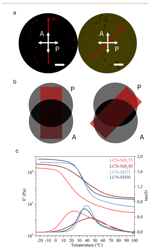
Fig. 2 Molecular alignment and mechanical tests on LCN films. (a) POM images of an LCN film with the director ( n ) oriented orthogonally to the polarisers and at 45°. Scale bar: 200 \mu\text{m} . (b) Schematization of the transmittance of LCN films under two crossed polarizer ( P ) and analyser ( A ). (c) Storage modulus ( E' ) and \tan(\delta) representative curves for the LCNs synthesised.
