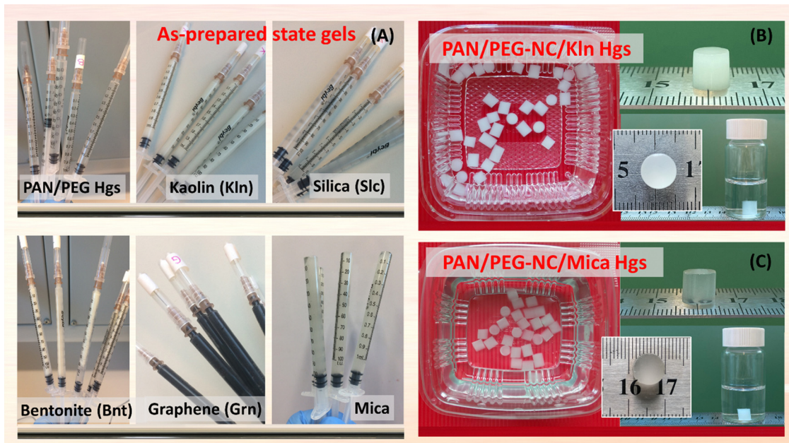
Scheme 2 Optical appearances of hybrid PAN/PEG-NC hydrogels containing various nanofillers after their preparation state (A), swollen-state view of Kln-integrated PAN/PEG-NC/Kln (B) and mica-integrated PAN/PEG-NC/Mica (C) hydrogels after swelling process.
