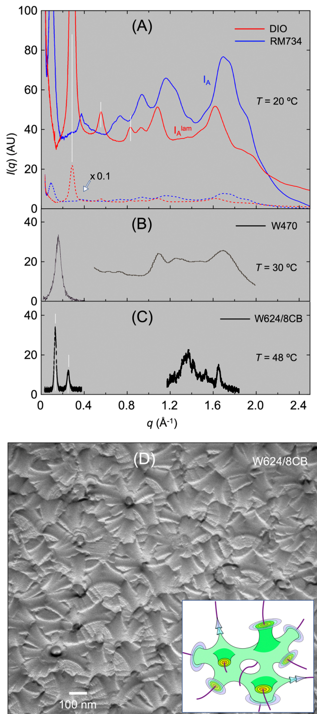
Fig. 7 Comparison of x-ray diffraction from the reentrant isotropic phases of RM734 and DIO with the scattering from other mesogenic systems that exhibit a reentrant isotropic phase and have similar X-ray diffraction signatures. (A) Full X-ray scans (SAXS + WAXS) of the I_R phase in RM734 and the I_R^{lam} phase in DIO, with the diffuse lamellar peaks in DIO indicated by white lines. (B) SAXS + WAXS scans of the reentrant isotropic phase of the single-component, chiral calamitic mesogen W470, from ref. 53. The molecule gels when dissolved, forming networks of nanoscale filaments, but the structure of the reentrant isotropic phase has not been visualized. (C) SAXS + WAXS scans of the reentrant isotropic phase of a 50/50 mixture of the bent-core mesogen W624 and 8CB. The white lines indicating the SAXS diffuse peak wavevectors are at q -values with the ratio 1 : 2, indicating that the local structure is lamellar (smectic-like), as in DIO.
