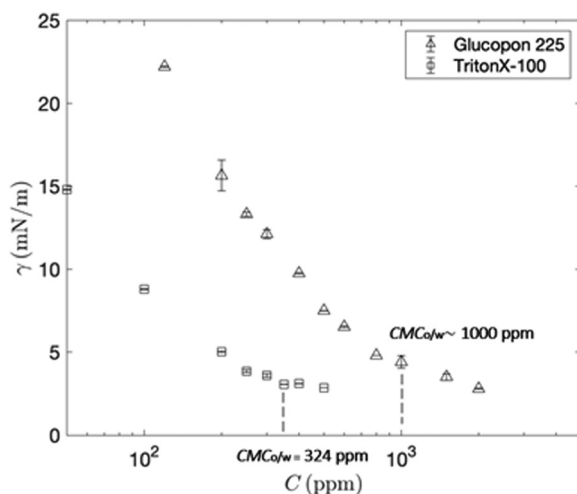
Fig. 6 IFT plotted as a function of surfactant concentration with both Triton X-100 (at equilibrium) and Glucopon 225 DK (at 10^3 \text{ s} , near equilibrium) for the LMO-in-water system. Error bars from replicates. CMC of each surfactants for oil–water emulsions are indicated.
