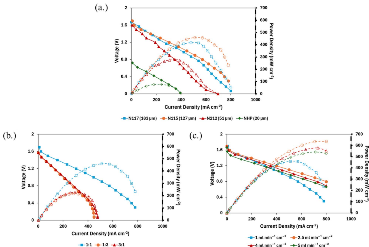
Fig. 4 Polarization and power density curve of the PMBI-DMHPFC with varying (a) membrane thickness (MeOH: 5 M, KOH: 3 M, H 2 O 2 : 5 M, H 2 SO 4 : 1.5 M, flow rate (anode and cathode): 1 ml min -1 cm -2 ), (b) flow rate ratio (MeOH: 5 M, KOH: 3 M, H 2 O 2 : 5 M, H 2 SO 4 : 1.5 M, membrane: N115, base flow rate: 1 ml min -1 cm -2 ), (c.) flow rate (MeOH: 5 M, KOH: 3 M, H 2 O 2 : 5 M, H 2 SO 4 : 1.5 M, membrane: N115).
