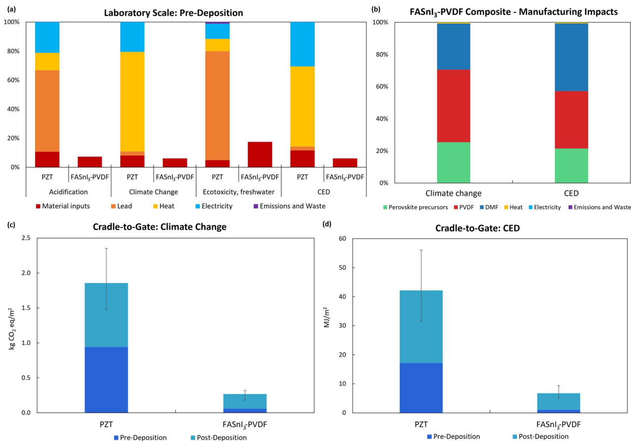
Fig. 4 Comparative cradle-to-gate environmental assessment of PZT and \text{FASnI}_3\text{-PVDF} composite: (a) impacts excluding the deposition stage; (b) contribution of individual sources to the environmental impacts of \text{FASnI}_3\text{-PVDF} ; and impacts including the deposition stage for (c) climate change and (d) cumulative energy demand (CED).
