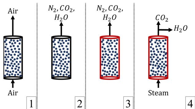
Fig. 1 Schematic representation of the four steps of the TVSA cycle: step 1—adsorption, during which ambient air enters the adsorption column. Step 2—evacuation, where residual gases are removed from the system until the desired desorption pressure is reached. Step 3—external heating, in which heat is supplied through a heating jacket (illustrated by red-coloured adsorption column walls) to raise the system temperature. Step 4—desorption, involving the continuous desorption of CO 2 and H 2 O, followed by the separation of these gases to improve CO 2 purity.
