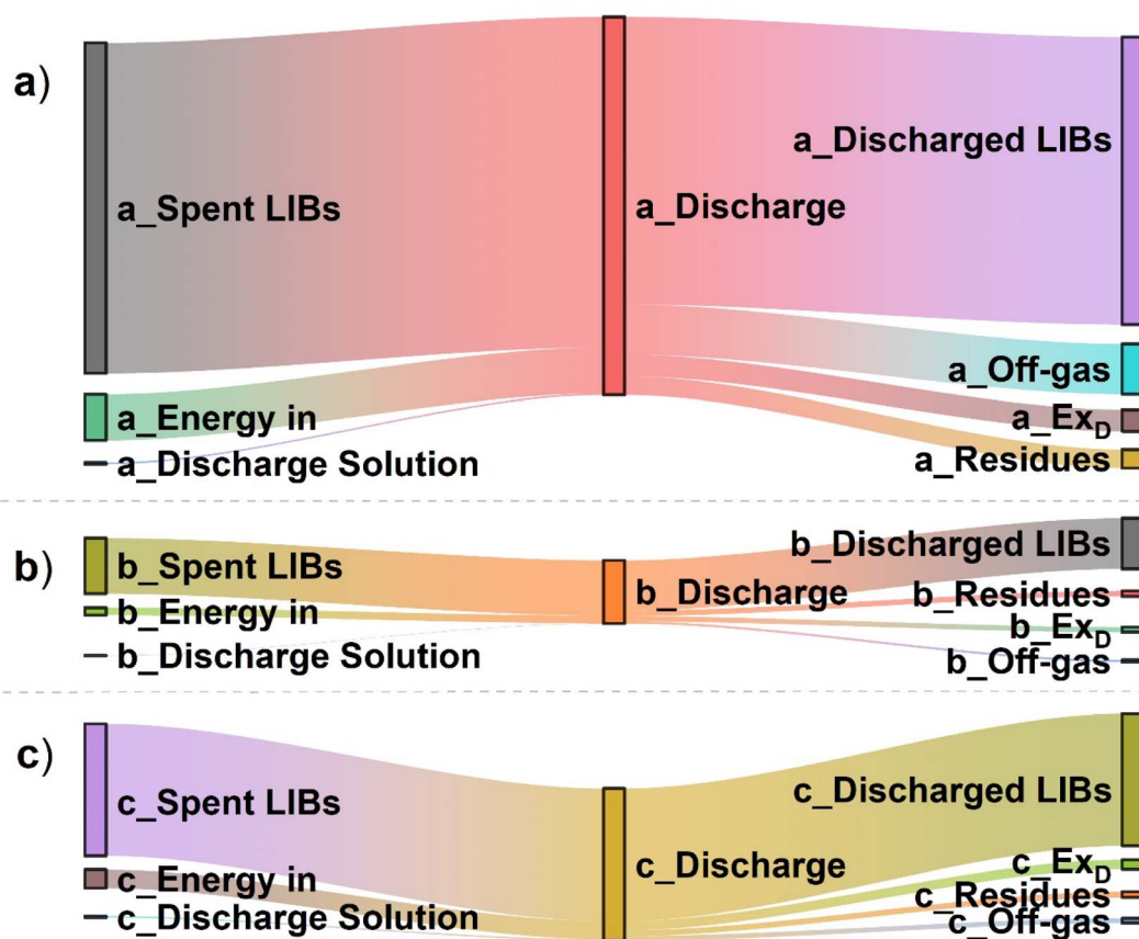
Fig. 4 The exergy content of each stream, with the input rate of spent LIBs in \text{kg h}^{-1} , for the three different discharge solutions: (a) NaCl, (b) \text{Na}_2\text{SO}_4 and (c) \text{Na}_2\text{CO}_3 .
