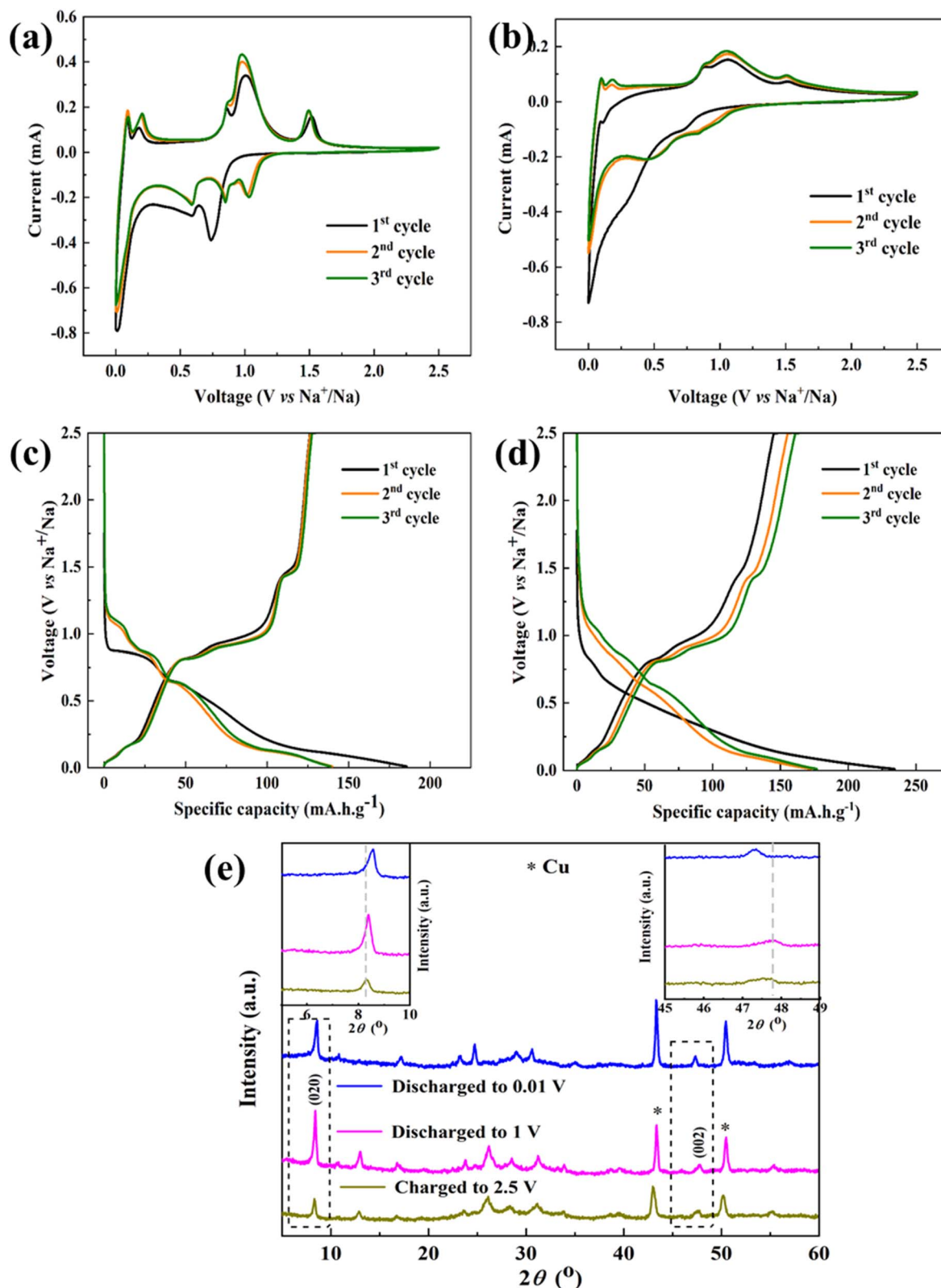
Fig. 4 Cyclic voltammety of (a) KNO and (b) KNO@F-C materials at a scan rate of 0.2 mV s -1 , and galvanostatic charge–discharge curves of (c) KNO and (d) KNO@F-C materials at a current density of 10 mA g -1 , for the first three cycles, and (e) ex situ XRD patterns of KNO@F-C electrode at various charge/discharge states (inset: enlarged view of (020) and (002) diffraction peaks).
