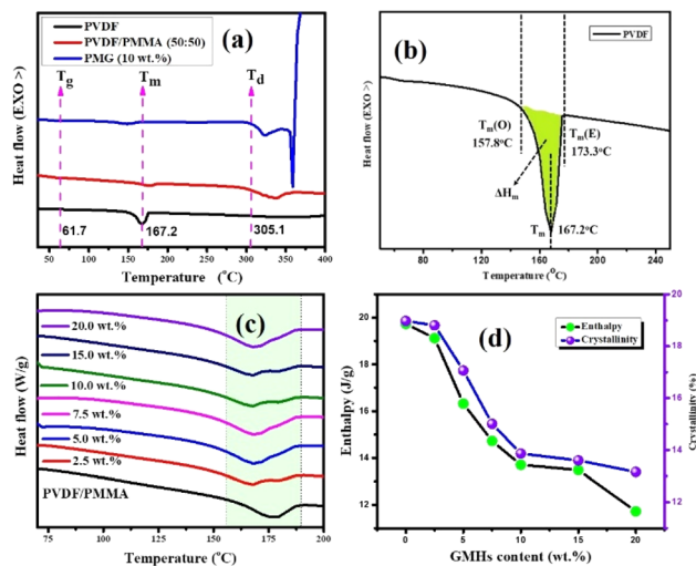
Fig. 4 DSC heating thermograms of (a) the 10 wt% GMH composite. (b) Onset melting temperature T_m(O) , peak melting temperature ( T_m ), end set temperature T_m(E) , change in melting enthalpy ( \Delta H_m ), and melting enthalpy ( \Delta H_m ) of pure PVDF. (c) DSC melting curves of the PVDF/PMMA-GMH composites and (d) melting enthalpy & crystallinity.
