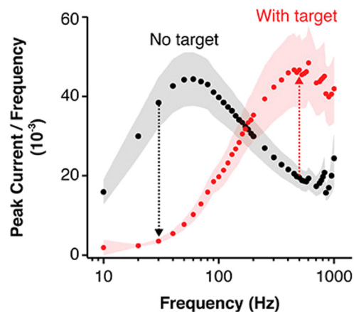
Fig. 10 E-AB sensors have an optimal interrogation frequency range irrespective of interrogation technique. Here, one can determine the frequency ranges in which the bound and un-bound probe aptamer each produces the highest faradic signal current. Reproduced from ref. 59 with permission from American Chemical Society, 59 copyright 2019.
