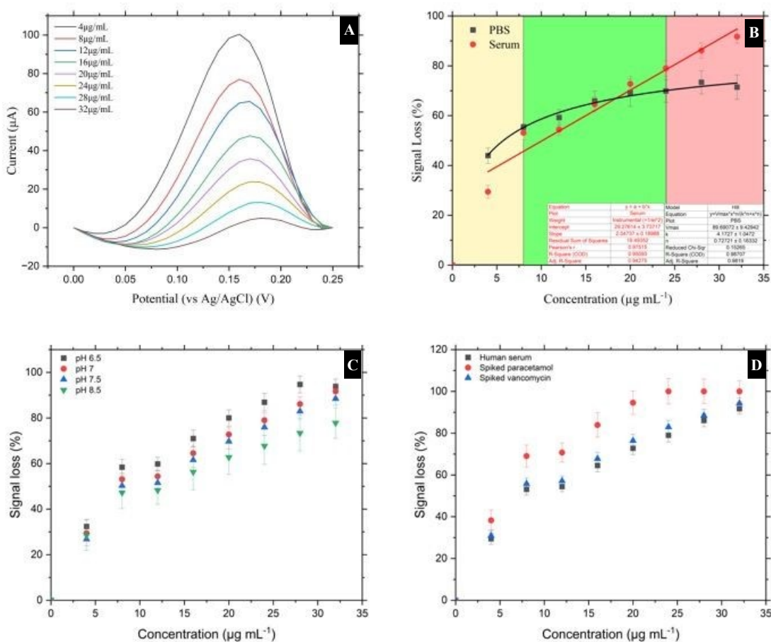
Figure 4: Analytical performance and specificity of the MIP-based RIF sensor. A) Differential Pulse Voltammetry (DPV) curves showing a concentration-dependent decrease in peak current with increasing concentrations of RIF in human serum. B) Calibration curves illustrating the sensor's response (% signal loss) to RIF in PBS versus spiked human serum, fitted with a non-linear Hill equation model. The highlighted green area indicates the therapeutic range for RIF (0 – 32 \mu\text{g mL}^{-1} ). C) Sensor stability analysis showing a consistent dose-response across a physiological pH range of 6.5 to 8.5. D) Specificity test demonstrating that the sensor's response to RIF is unaffected by the presence of potential interferent, vancomycin, in spiked human serum. However, an interference from paracetamol was observed, saturating the sensor at 24 \mu\text{g mL}^{-1} . Such an interference can be dealt with integration of machine learning (ML) models which can potentially attenuate the effects of interference. A multiple input single output (MISO) model can potentially improve the sensor performance in complex matrices by using multiple feature to predict the concentration more accurately.
