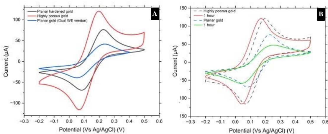
Figure 2A) Cyclic voltammogram comparing the older dual working electrode design (planar gold) to the newer quad-working planar and HPG. B) Cyclic voltammogram comparing the biofouling resistance of the HPG to planar gold.
