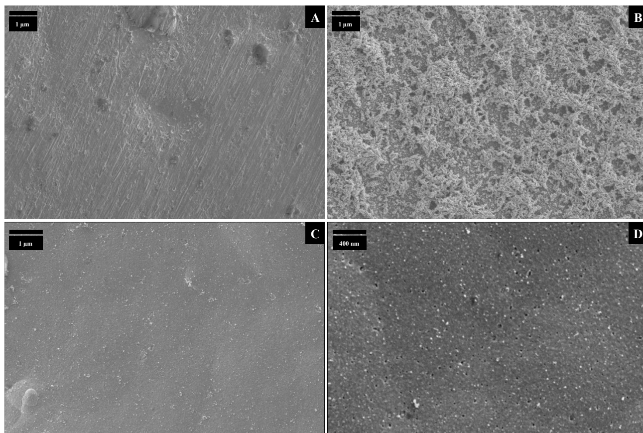
Figure 3 Surface characterization: Scanning Electron Micrographs (SEM) A) SEM image of planar gold. B) SEM image of highly porous gold electrode. C) SEM image of molecularly imprinted polymer (MIP) on planar gold electrodes. D) SEM image of molecularly imprinted polymer on planar gold electrodes.
