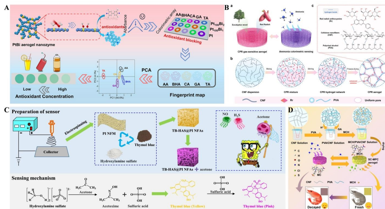
Fig. 12 (A) Schematic representation of the Pt-Bi aerogel-based colorimetric sensor array for the discrimination of antioxidants. Reproduced with permission from ref. 176 . Copyright 2025, Elsevier. (B) Synthesis of poly(vinyl alcohol) and nanocellulose-based bio-aerogel for the colorimetric determination of ammonia. Reproduced with permission from ref. 177 . Copyright 2024, American Chemical Society. (C) Development of 3D polyimide aerogel for the colorimetric detection of breath acetone. Reproduced with permission from ref. 178 . Copyright 2024, Elsevier. (D) Schematic representation of the synthesis of sulfonated spirocyclic pyran aerogel for the visual detection of ammonia. Reproduced with permission from ref. 173 . Copyright 2025, Elsevier.
