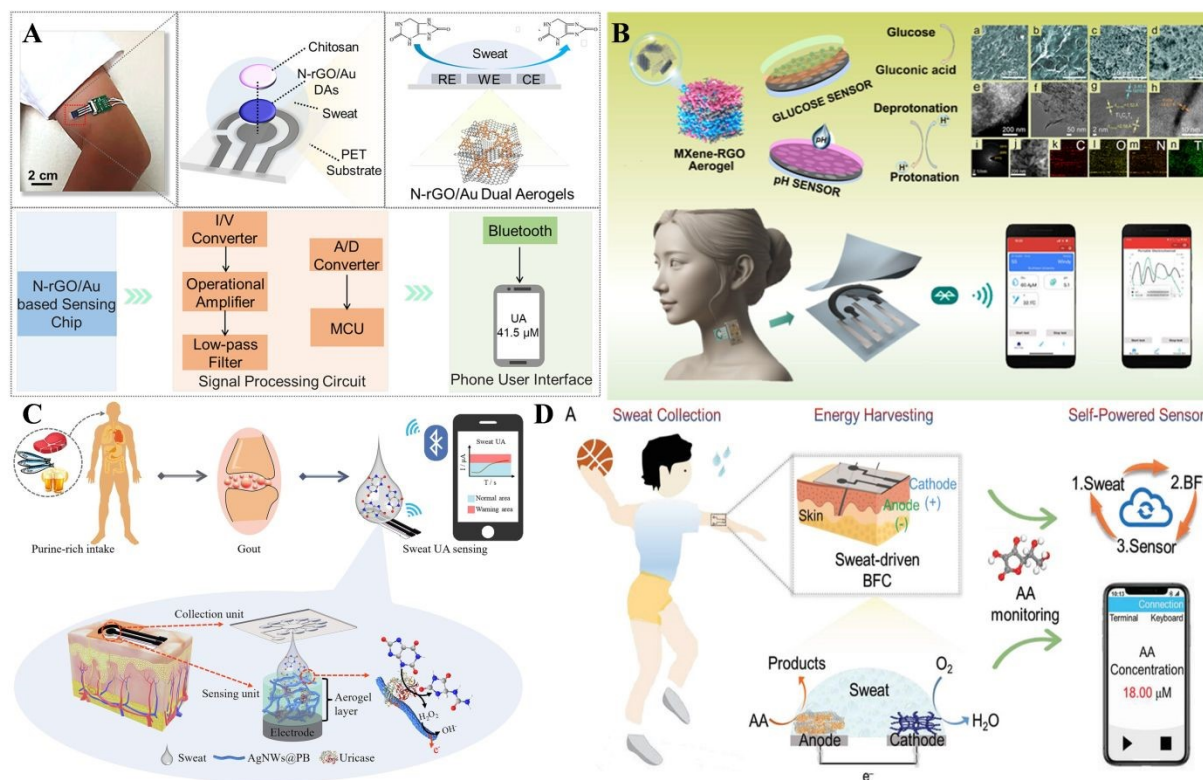
Fig. 8 (A) Schematics and working principle of N-Doped reduced graphene oxide/Au aerogels based nonenzymatic wearable uric acid sensor. Reproduced with permission from ref. 64 Copyright 2023, American Chemical Society. (B) Schematic illustration of the construction and working principle of the 3D Graphene MXene aerogel-based integrated sweat glucose monitoring sensor. Reproduced with permission from ref. 125 Copyright 2024, American Chemical Society. (C) Illustration of wearable non-invasive dynamic monitoring of sweat uric acid based on silver nanowires@Prussian blue-aerogel. Reproduced with permission from ref. 63 Copyright 2024, Elsevier. (D) Illustration of metal-aerogel-based wearable biofuel cells for energy harvesting, sweat collection, and biosensor. Reproduced with permission from ref. 127 Copyright 2024, Wiley-VCH GmbH.
